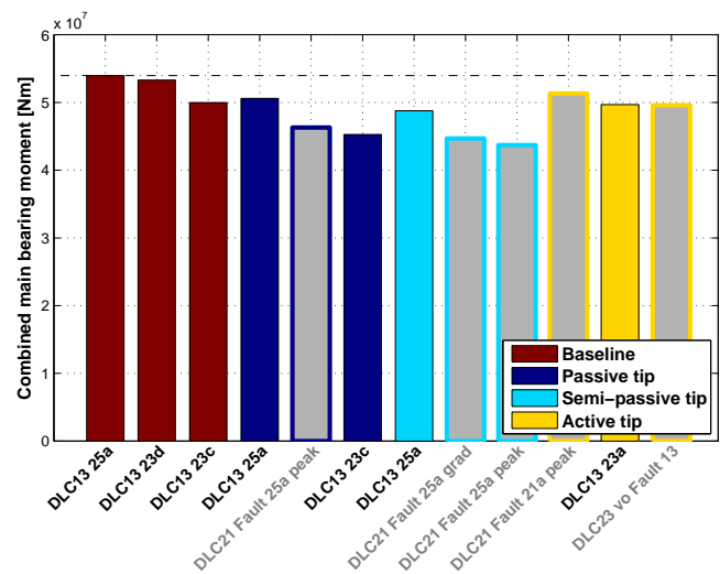
Figure 12. Ranking analysis of main bearing combined moment. Blade tip fault conditions are displayed using gray-shaded bars.
