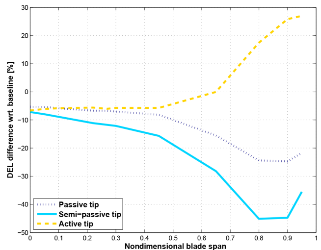
Figure 9. Top: percent variation of DELs at verification spots. Bottom: percent variation of DELs vs. blade span.
