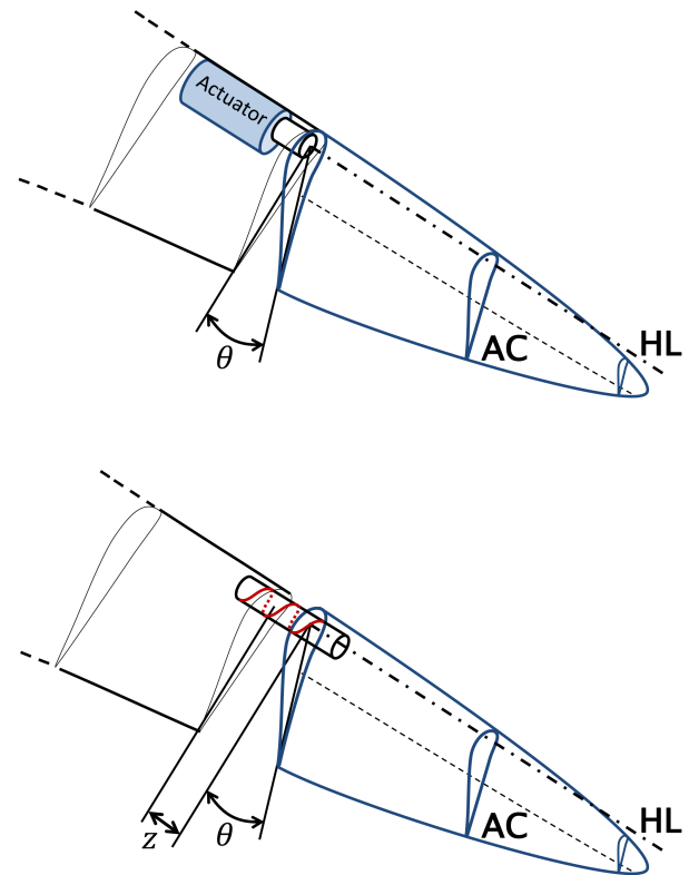
Figure 3. Top: semi-passive tip configuration. Bottom: passive tip configuration.
