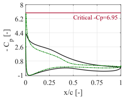
(b) M_\infty = 0.3
