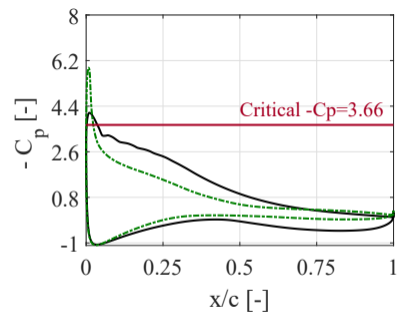
(c) M_\infty = 0.4
