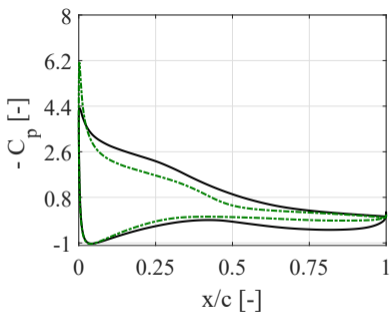
(a) M_\infty = 0.2
