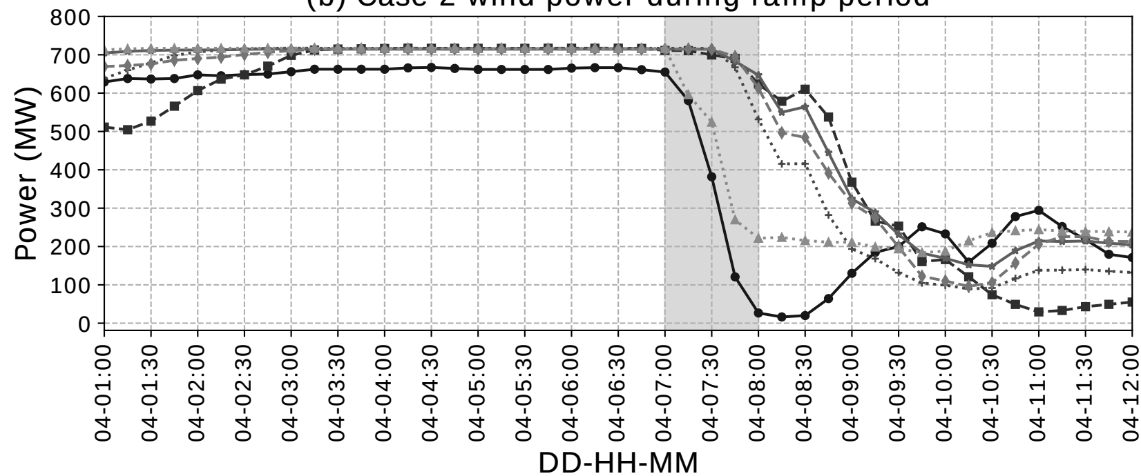
(b) Case 2 wind power during ramp period
