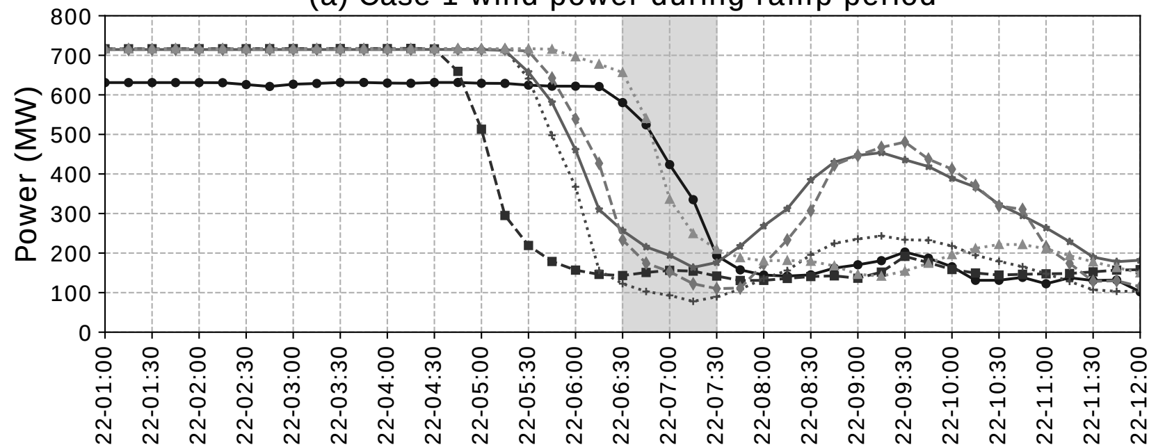
(a) Case 1 wind power during ramp period
