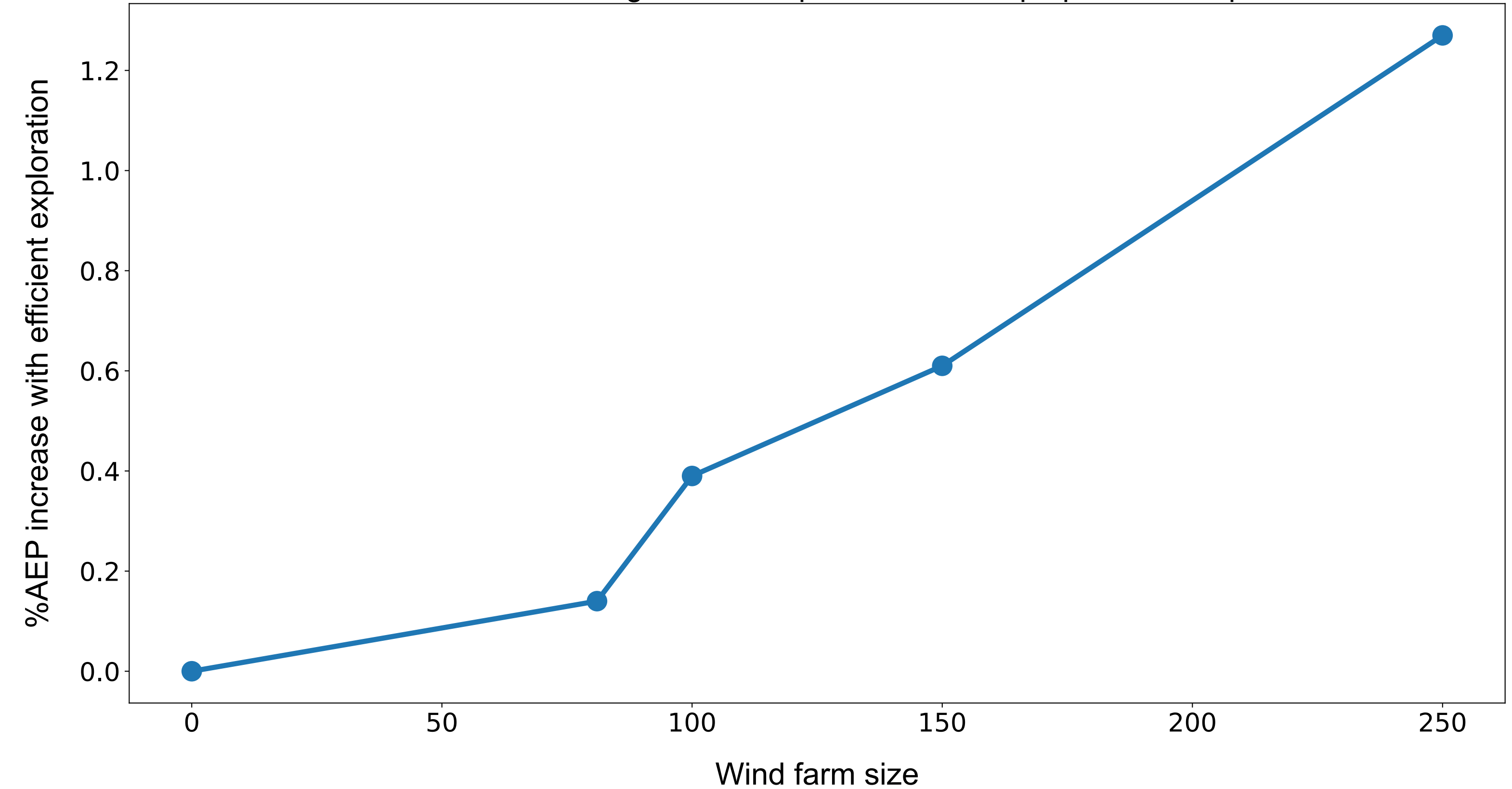
% AEP increase when using efficient exploration for shape parameter optimization
