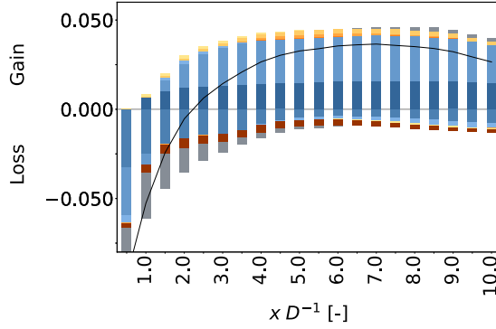
(b) wake steering
