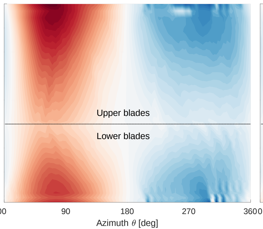
XFOIL Re = 80K Ncrit = 4 50%
