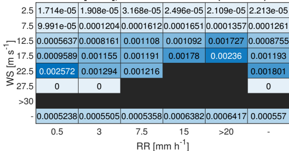
F/R [1/mm], meas. GEHALX 2022 (n = 28538)
