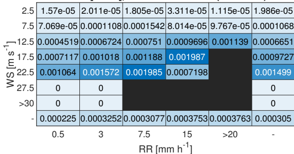
F/R [1/mm], meas. EWTW 2022 (n = 45558)
