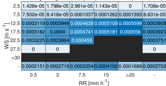
F/R [1/mm], ASPIRE (LES) EWTW 2022 (n = 105522)
