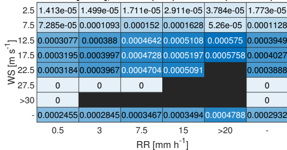
F/R [1/mm], ASPIRE (LES) LEG 2022 (n = 70916)
