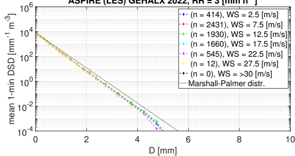
ASPIRE (LES) GEHALX 2022, RR = 3 [mm h -1 ]
