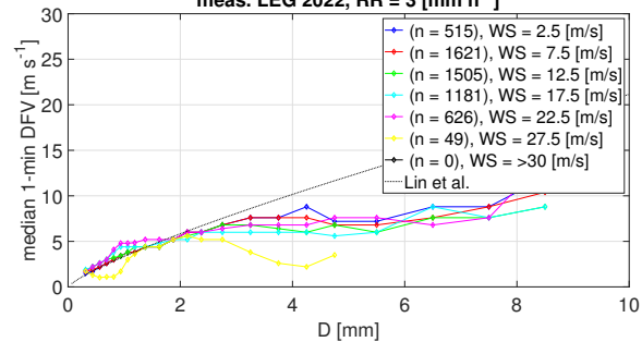
meas. LEG 2022, RR = 3 [mm h -1 ]
