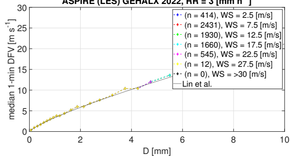
ASPIRE (LES) GEHALX 2022, RR = 3 [mm h -1 ]
