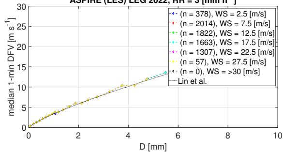
ASPIRE (LES) LEG 2022, RR = 3 [mm h -1 ]
