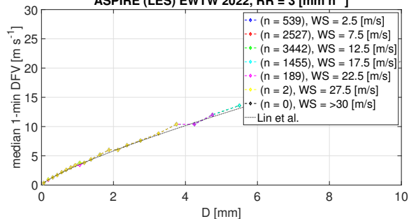
ASPIRE (LES) EWTW 2022, RR = 3 [mm h -1 ]
