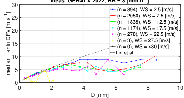
meas. GEHALX 2022, RR = 3 [mm h -1 ]
