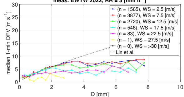
meas. EWTW 2022, RR = 3 [mm h -1 ]
