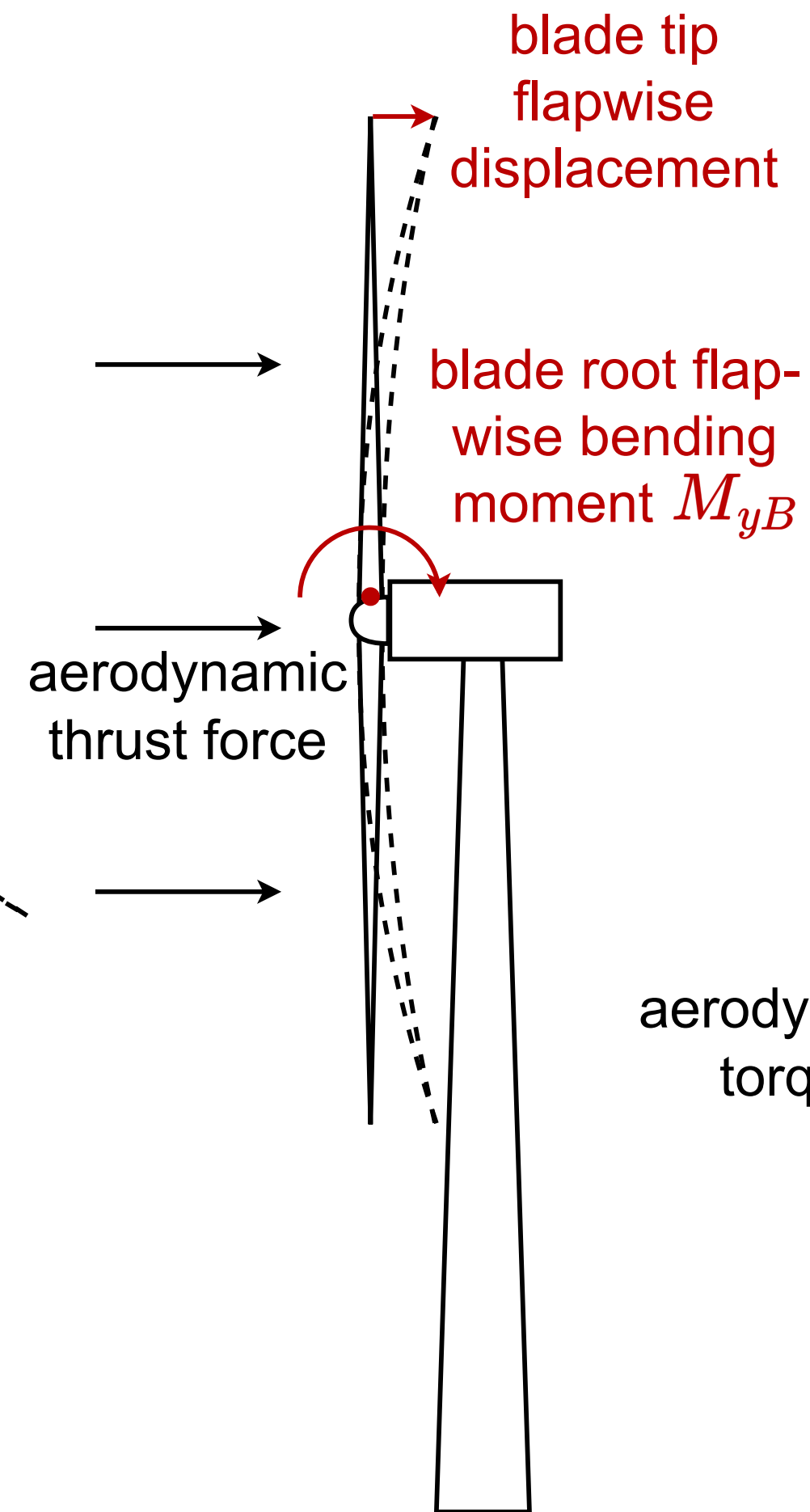
Blade flapwise
