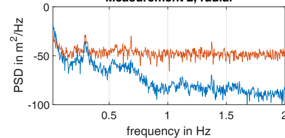
Measurement 2, radial
