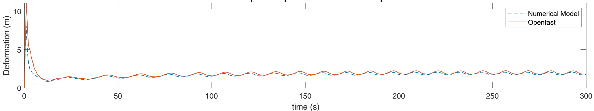
Blade tip out-of-plane deformation at 7mps
