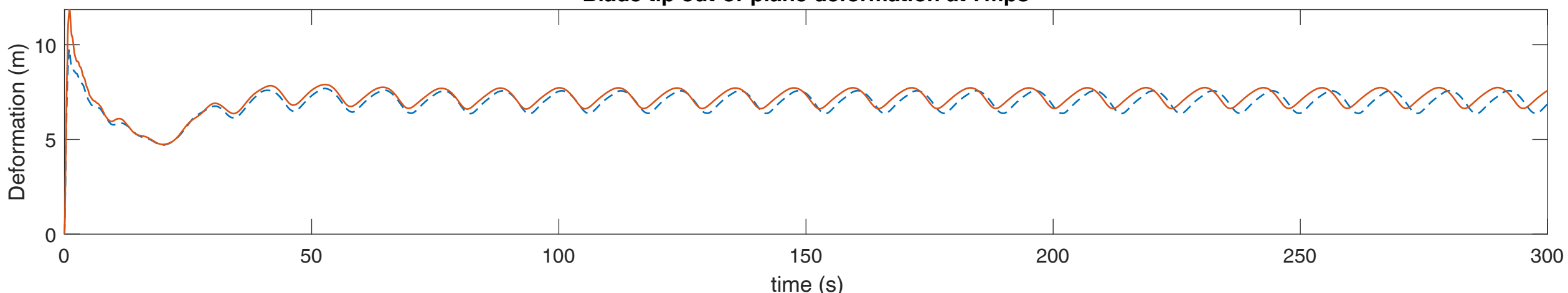
Blade tip out-of-plane deformation at 9mps
