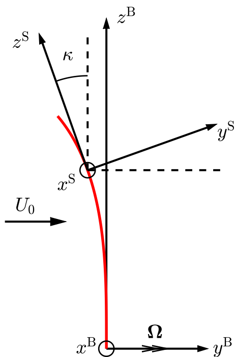
(a) upwind prebend
