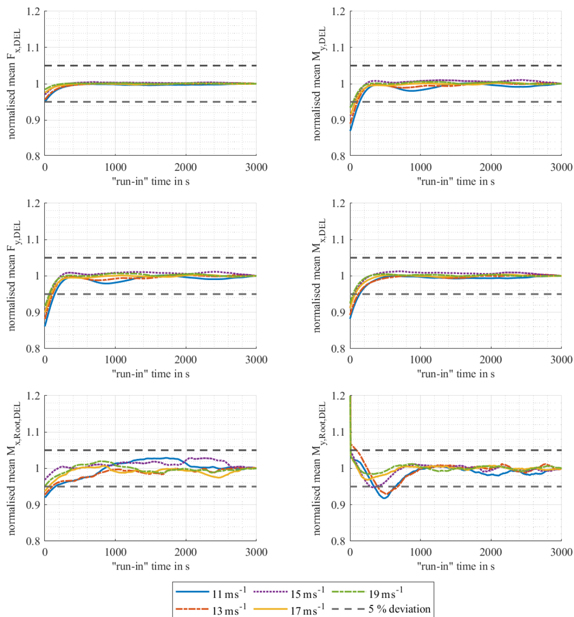
Figure A2. Initial transient behaviour of the idling wind turbine for mean wind speeds of 11 to 19 \text{m s}^{-1} for all considered internal forces.
