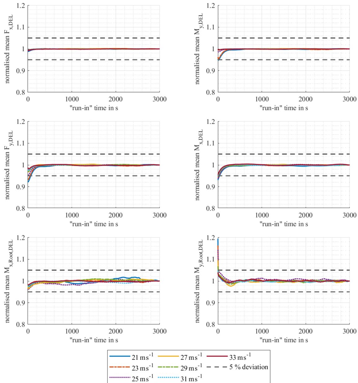
Figure A3. Initial transient behaviour of the idling wind turbine for mean wind speeds of 21 to 33 m s −1 for all considered internal forces.
