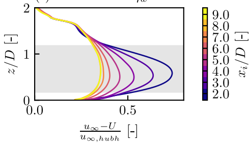
(f) H300-C8-G1 \eta_w = 1.00
