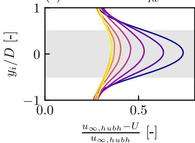
(e) H300-C8-G1 \eta_w = 1.00
