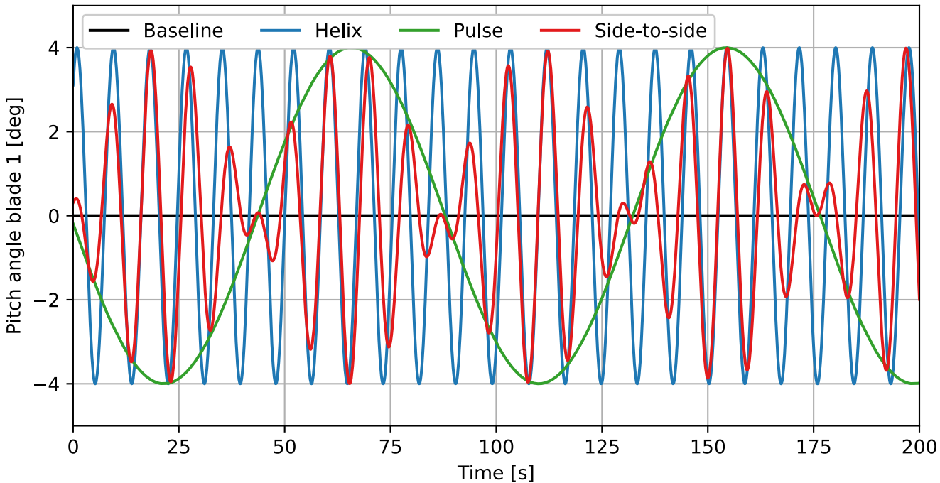
Pitch actuation for different control strategies
