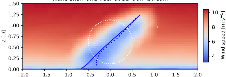
Wake skew and veer at 5D downstream
