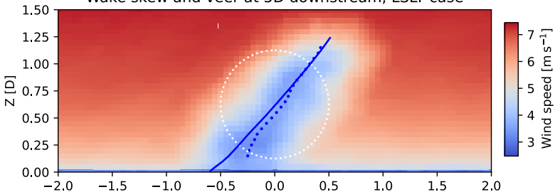
Wake skew and veer at 5D downstream, LSLT case
