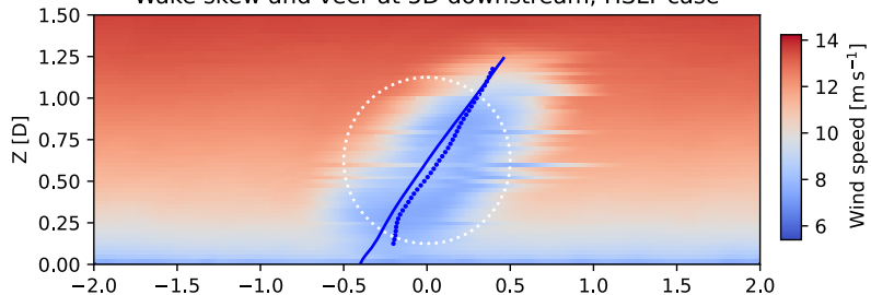
Wake skew and veer at 5D downstream, HSLT case
