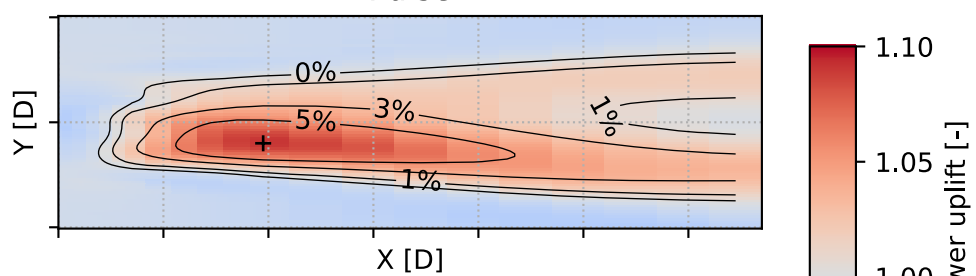
Wake steering
