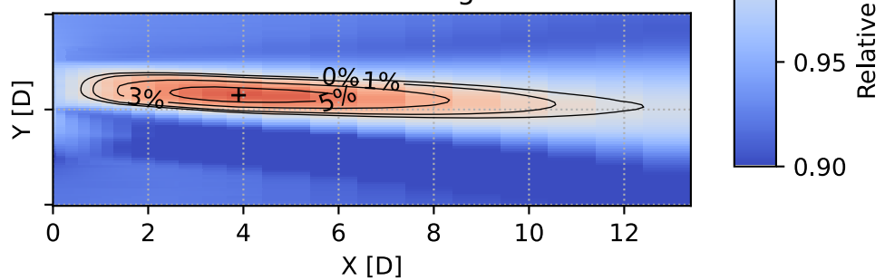
Wake steering
