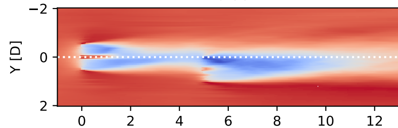
Wake steering
