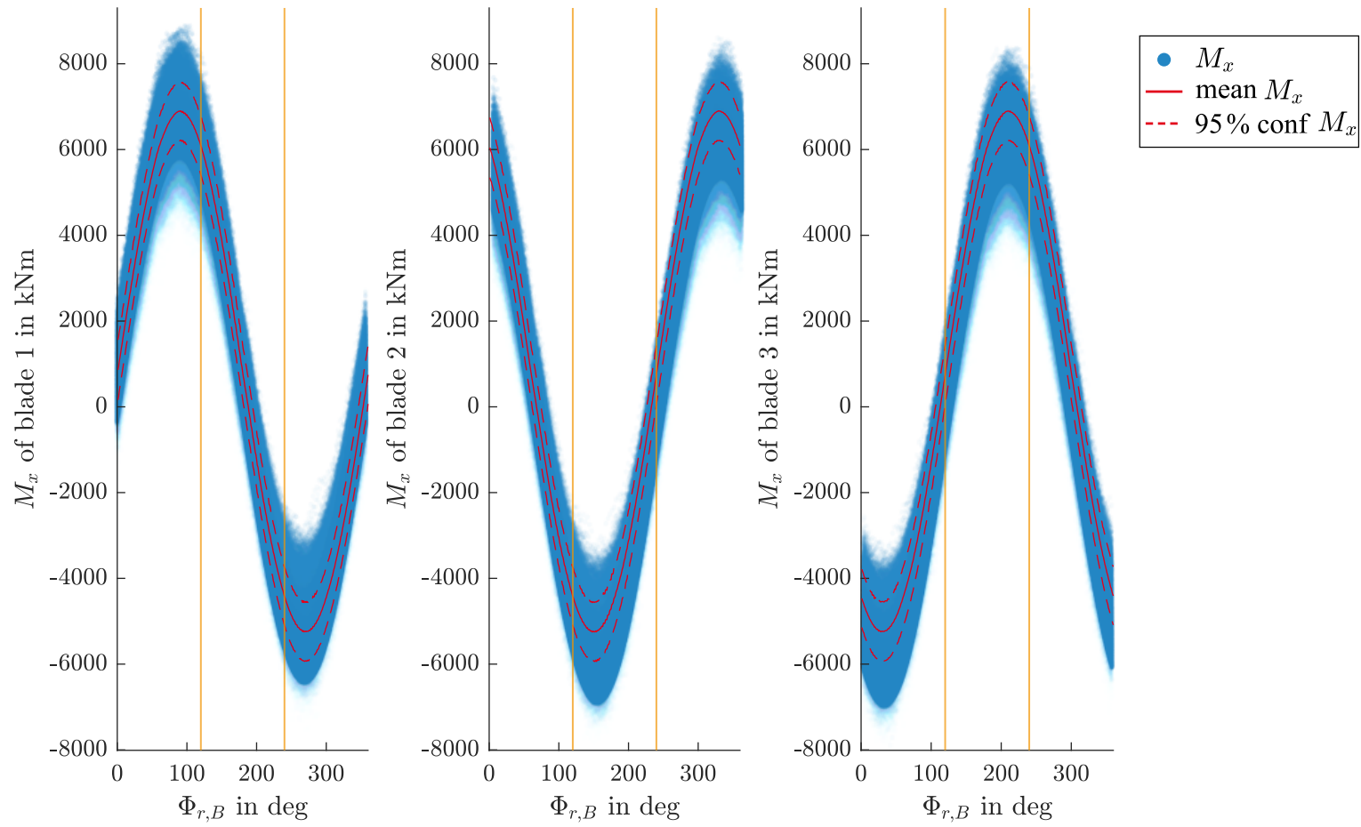
Weighted M_x over \Phi_{r,B} of simulation data
