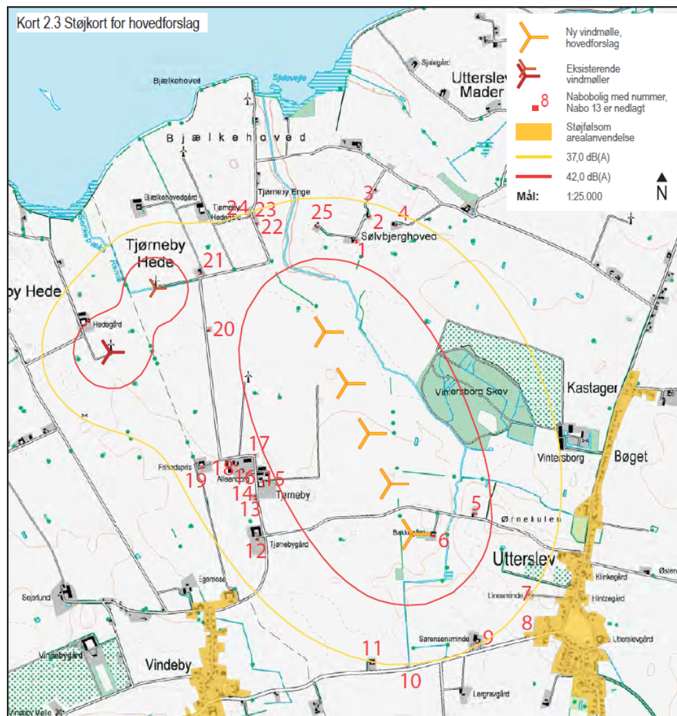
Figure 1. Example of a noise contour map (from Tjørneby wind farm EIA, 2011).
