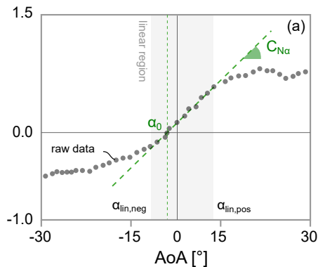
normal force coefficient ( C_n )
