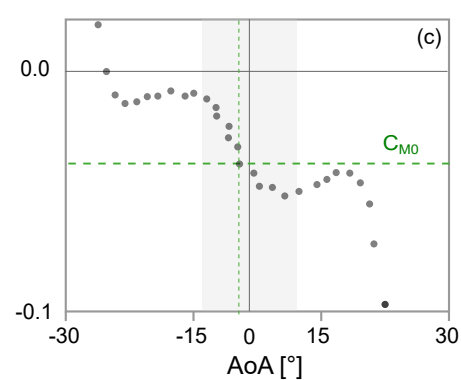
pitching moment coefficient ( C_m )
