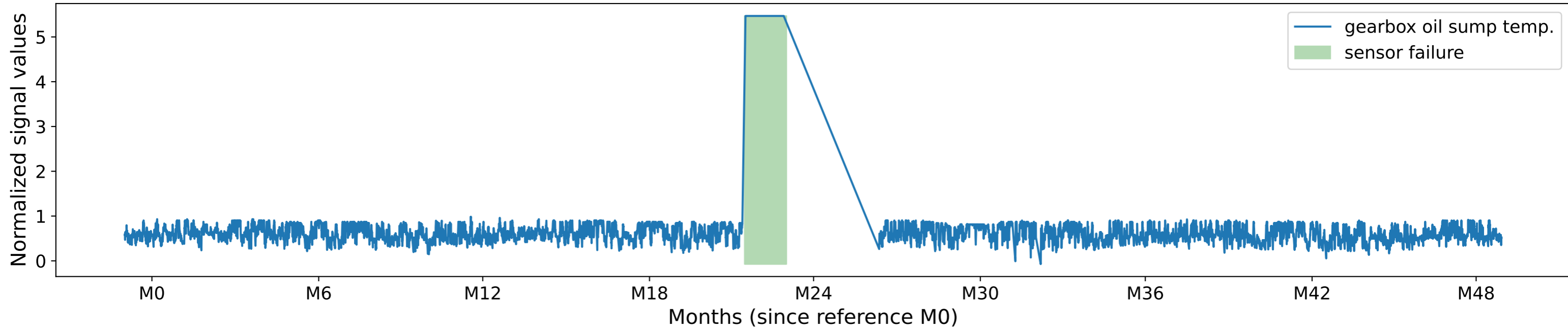
Signal with sensor error: gearbox oil sump temp. (normalized)
