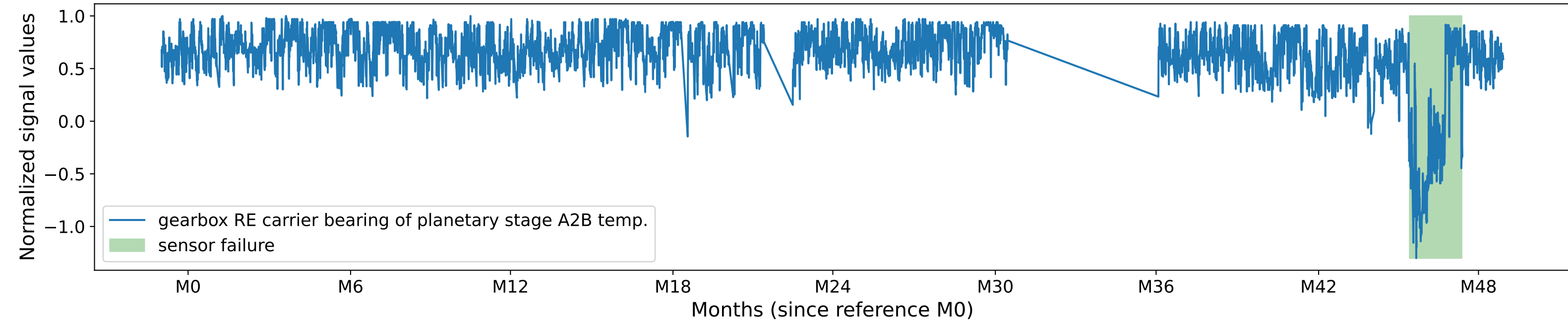
Signal with sensor error: gearbox RE carrier bearing of planetary stage A2B temp. (normalized)
