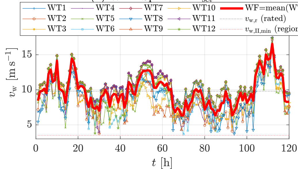
(c) Physical Inertia for P_{\text{set}} = 1
