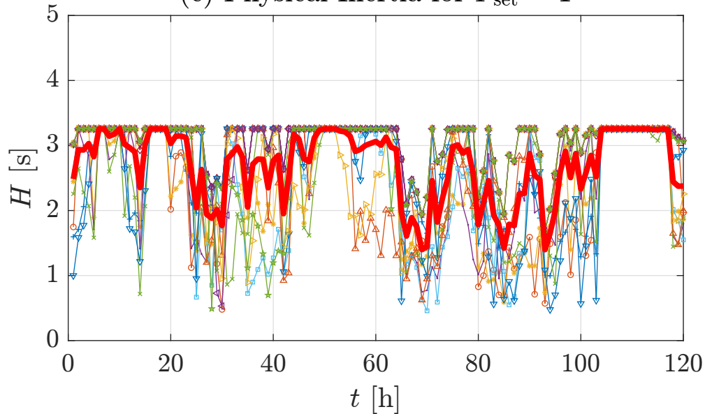
(c) Physical Inertia for P_{\text{set}} = 1
