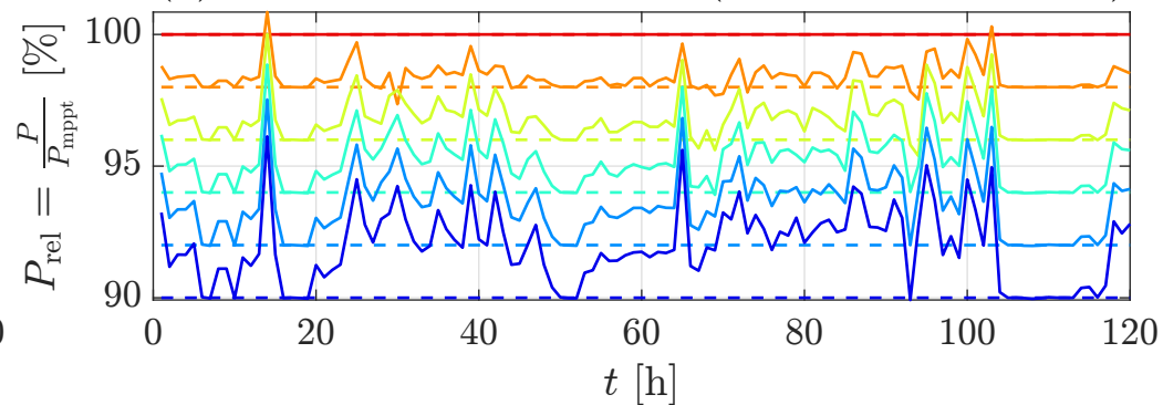
(f) Max. Virtual Inertia
