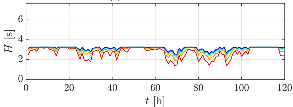
(e) Physical Inertia
