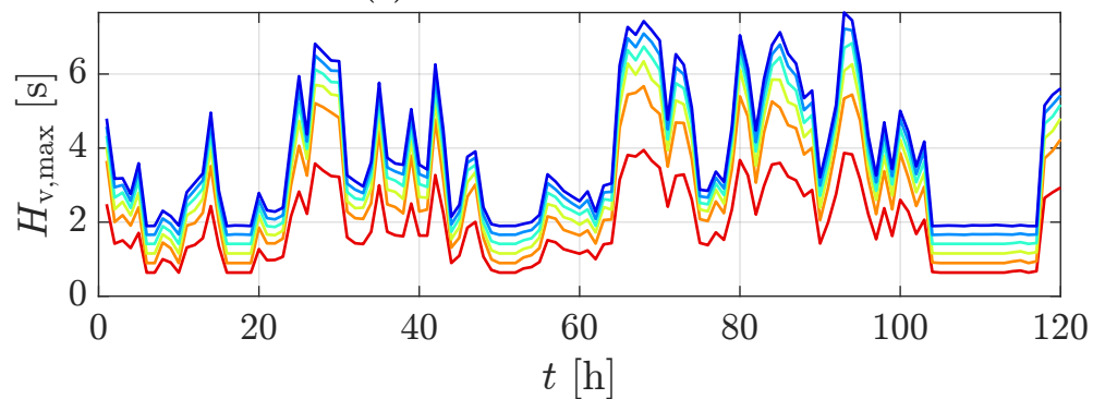
(f) Max. Virtual Inertia
