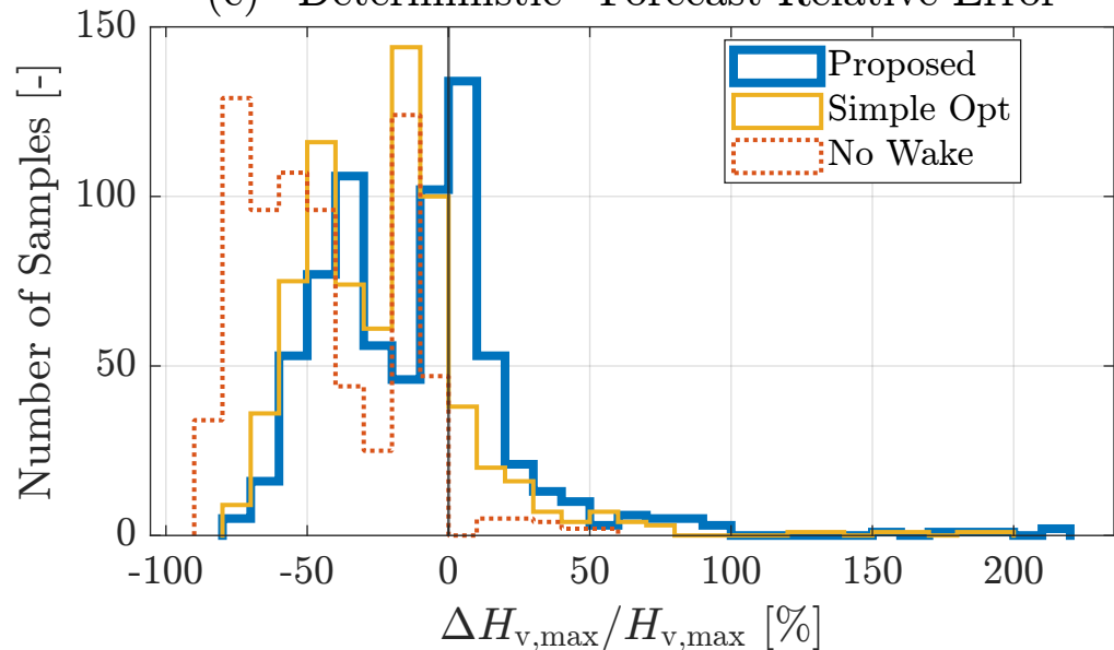
(c) “Deterministic” Forecast Relative Error
