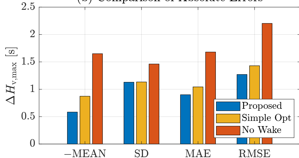
(b) Comparison of Absolute Errors
