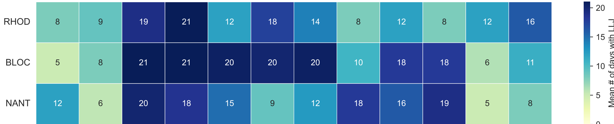
Average Number of Days with LLJ
