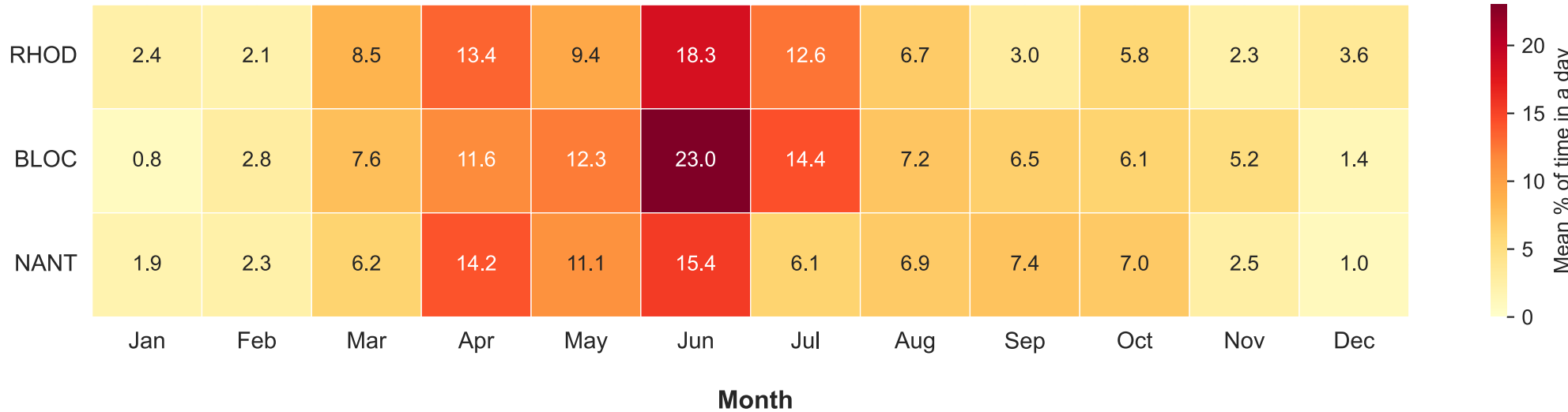
Monthly Mean Frequency of LLJ Occurrence
