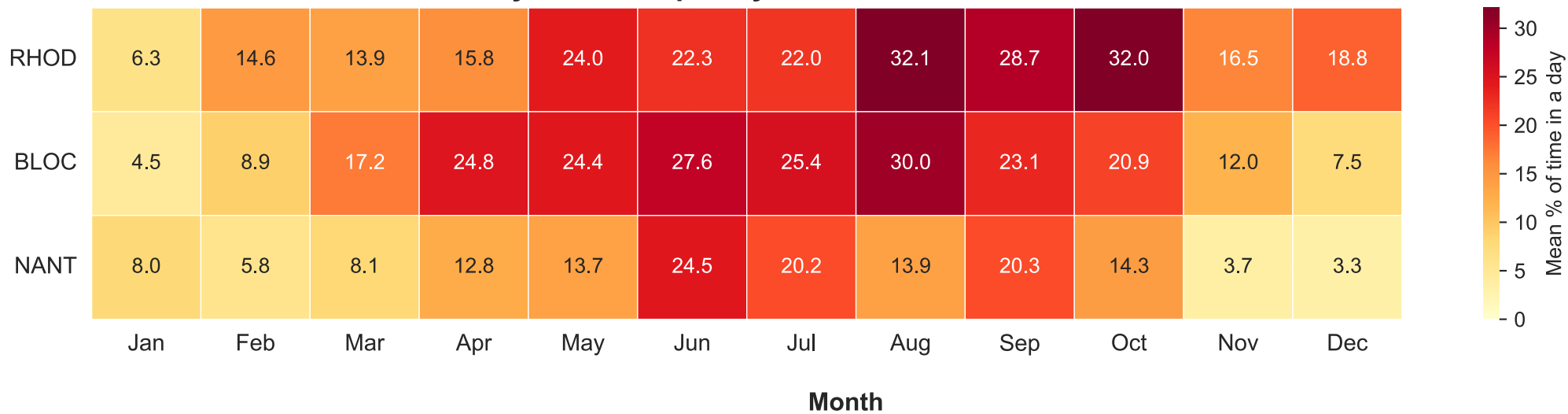
Monthly Mean Frequency of Extreme Wind Veer
