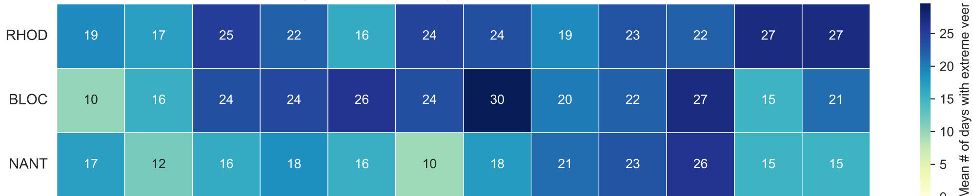
Average Number of Days with Extreme Wind Veer
