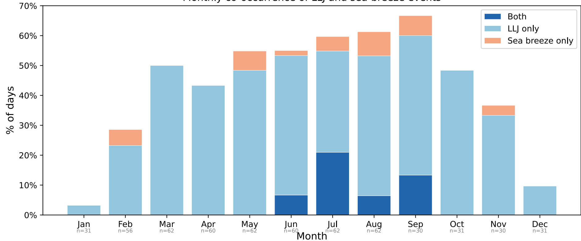
Monthly co-occurrence of LLJ and sea-breeze events
