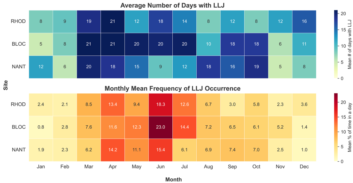
Figure 4. Monthly low-level jet (LLJ) characteristics at three WFIP3 sites (RHOD, BLOC, NANT) from February 2024 to August 2025. The top panel shows the average number of days per month with an LLJ detected from the lidar data, and the bottom panel shows the mean percentage of time in a day an LLJ is detected for each month and site.
