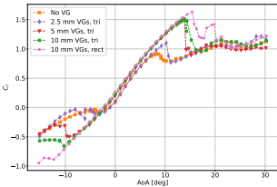
(a) Lift Coefficient
