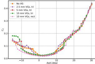
(b) Drag Coefficient
