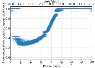
(c) No VGs, k = 0.018
