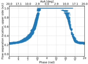
(a) No VGs, k = 0.045
