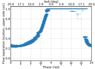
(b) No VGs, k = 0.09
