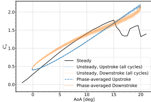
(b) 10 mm VGs, rectangular vanes, k = 0.09
