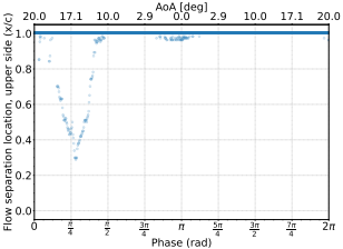
(a) 10 mm VGs, rectangular vanes, k = 0.045
