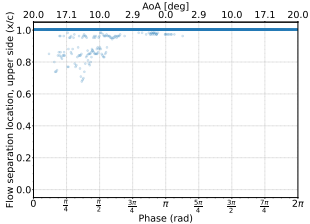
(b) 10 mm VGs, rectangular vanes, k = 0.09
