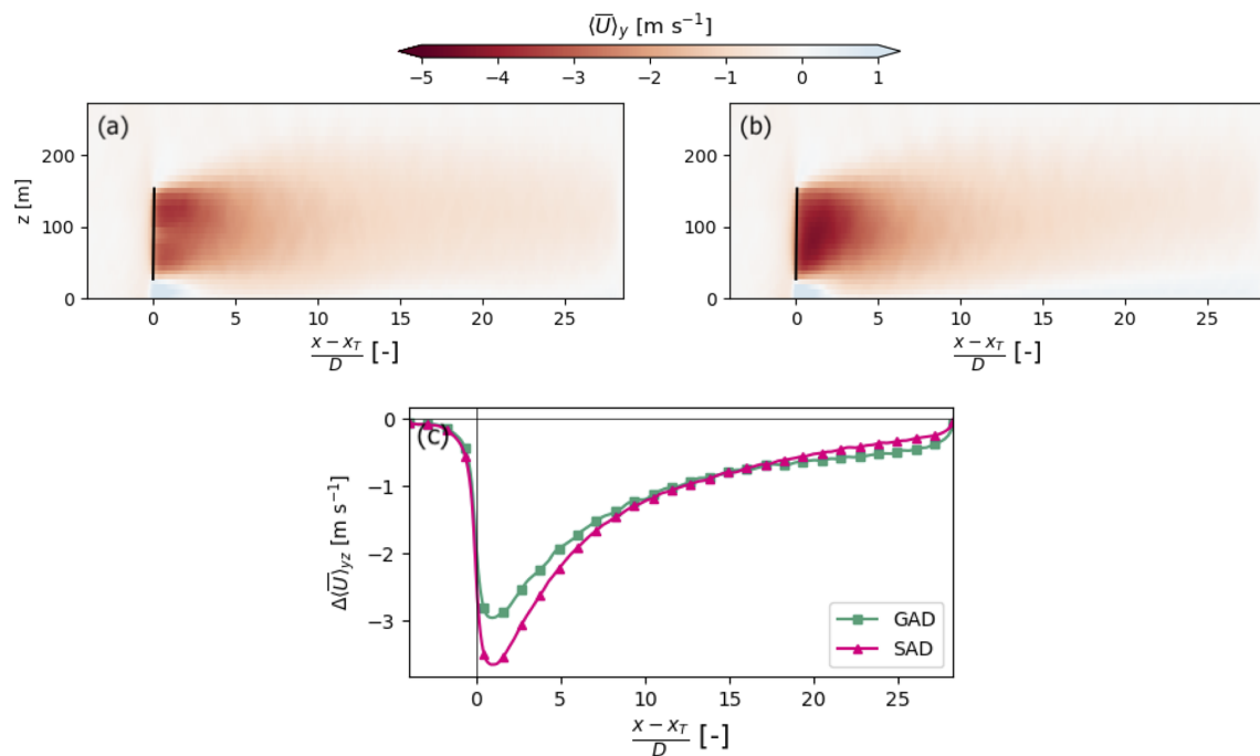
Figure B4. Time- and space-averaged wind speed deficit for the GAD (a) and SAD (b) wind turbine parameterizations at the turbine location. The rotor-averaged wind speed deficit is shown in panel (c). The velocity fields in panels (a) and (b) are averaged along the y direction across the turbine diameter. The rotor-averaged velocity field in panel (c) is also averaged vertically across the turbine rotor layer.
