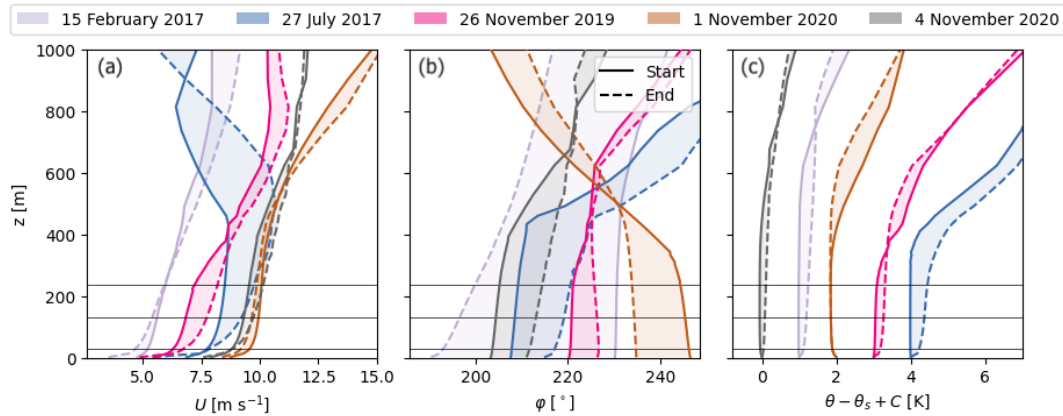
Figure 3. Vertical profiles of wind speed (a), wind direction (b), and potential temperature (c) for the five simulated dates. For each date, the first and last valid time stamps are represented by the solid and dashed lines, respectively, while time stamps in between are represented by the filled colors. The horizontal black lines in each panel represent the bottom of the rotor, hub height, and top of the rotor for the 11 MW wind turbine.
