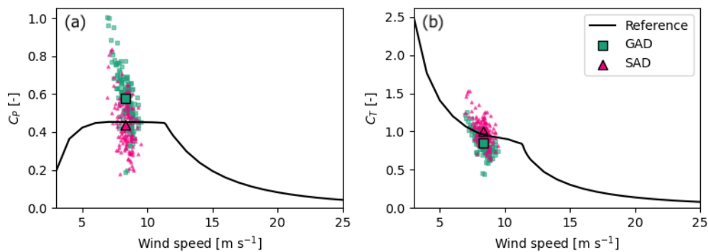
Figure B2. Power (a) and thrust (b) coefficient curves for the NREL 5 MW wind turbine. The instantaneous results are shown in green for the GAD and in magenta for the SAD. The large colored symbols with black edges in each panel represent the mean over the simulated time period.
