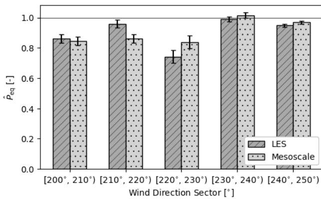
Figure 17. Normalized equivalent wind turbine power across the three wind farms for each wind direction sector for the mesoscale simulation and LES. The error bars represent the 95% confidence interval in the data.
