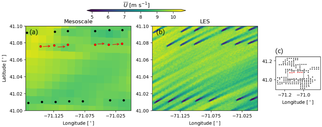
Figure 14. Time-averaged velocity field at hub height for the mesoscale simulation (a) and LES (b) on 1 November 2020 at 12:52 UTC. The mean wind direction at hub height is 245^\circ . Panel (c) shows the region considered in panels (a) and (b). Front-row turbines in South Fork and Revolution Wind waking their neighbors are highlighted with the red circles in panels (a) and (c).
