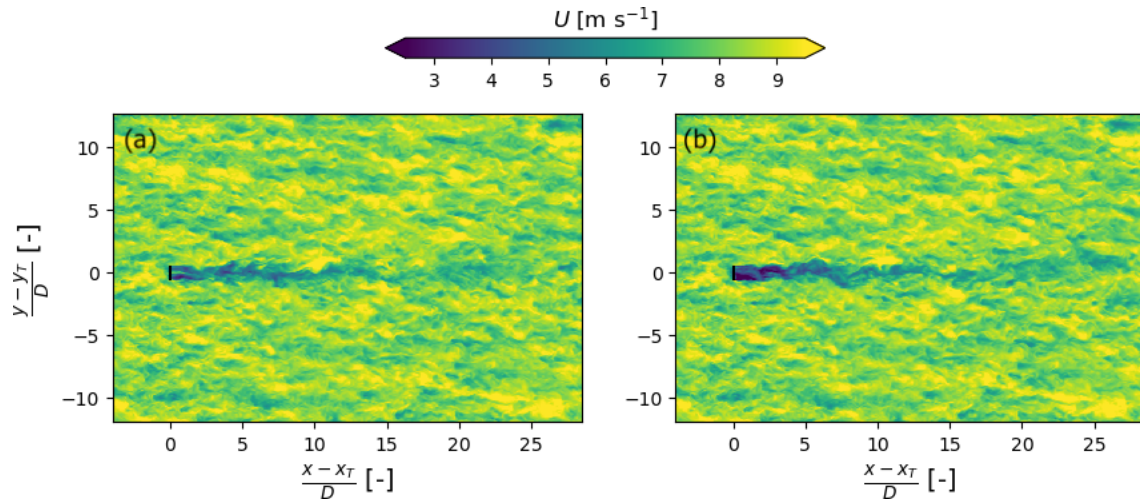
Figure B3. Instantaneous hub-height wind speed for the GAD (a) and SAD (b) wind turbine parameterizations. The location of the turbine is represented by the solid black line. The x and y axes are normalized to represent the distance in rotor diameters ( D ) from the turbine parameterization.
