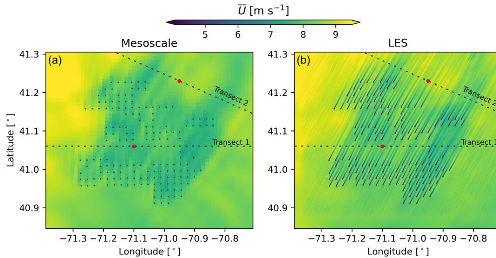
Figure 6. Time-averaged velocity field at hub height for the mesoscale simulation (a) and LES (b) on 4 November 2020 at 20:37 UTC. The dotted black lines in each panel illustrate the locations of the velocity transects, and the red dots indicate the midpoint distance of each transect.
