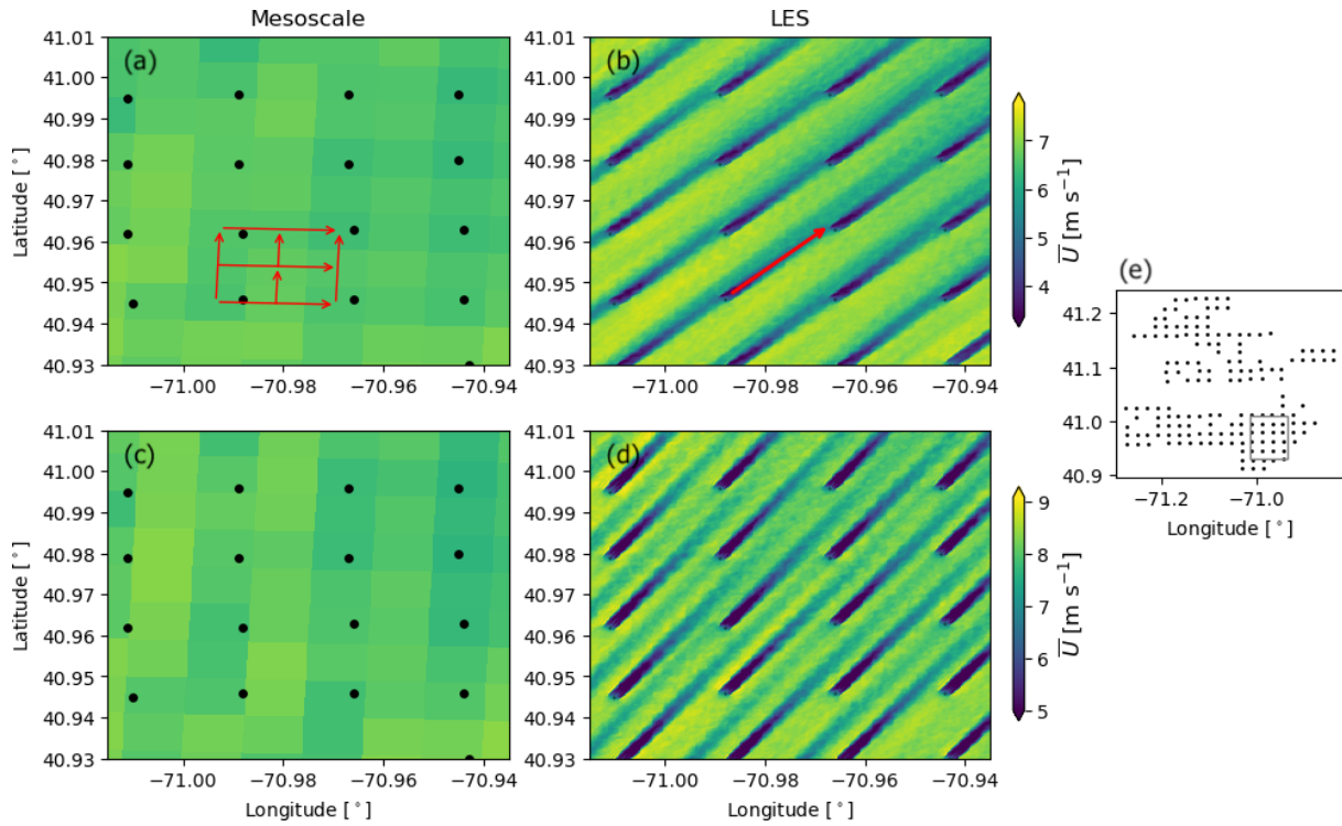
Figure 16. Time-averaged velocity field at hub height for the mesoscale simulation (a, c) and LES (b, d) on 26 November 2019 at 15:52 UTC (a, b) and 28 July 2017 at 00:07 UTC (c, d). The mean wind direction at hub height is 221° on 26 November 2019 at 15:52 UTC and 212° on 28 July 2017 at 00:07 UTC. Panel (e) illustrates the region shown in panels (a)–(d). The red arrows in panels (a) and (b) illustrate the predominant wake propagation direction in each modeling framework.
