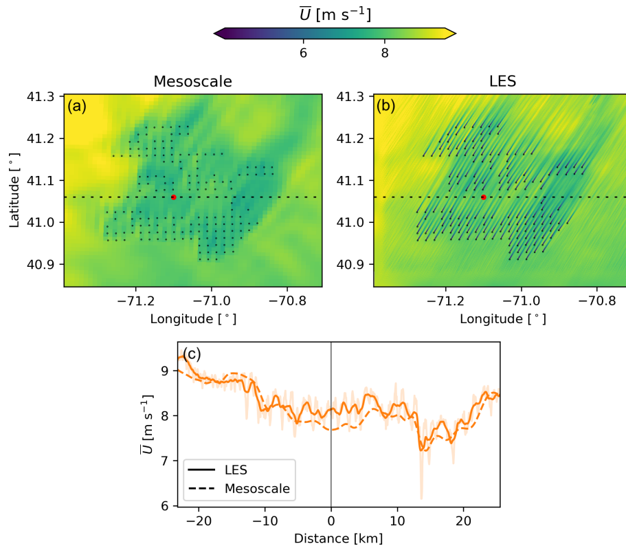
Figure 8. Time-averaged velocity field at hub height for the mesoscale simulation (a) and LES (b) under unstable atmospheric conditions. The velocity fields are averaged in time between 22:00 and 22:15 UTC on 27 July 2017. The dotted black lines in each panel illustrate the locations of the velocity transects, and the red dots indicate the midpoint distance of each transect. Panel (c) shows the velocity along the transect for the LES and mesoscale simulation. For reference, the mean wind direction across the region is 208^\circ .
