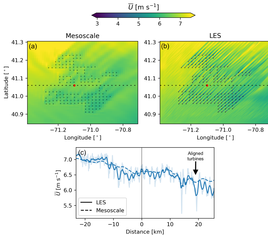
Figure 7. Time-averaged velocity field at hub height for the mesoscale simulation (a) and LES (b) under stable atmospheric conditions. The velocity fields are averaged in time between 14:30 and 14:45 UTC on 26 November 2019. The dotted black lines in each panel illustrate the locations of the velocity transects, and the red dots indicate the midpoint distance of each transect. Panel (c) shows the velocity along the transect for the LES and mesoscale simulation. For reference, the mean wind direction across the region is 219°.
