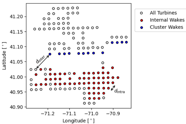
Figure 11. Wind turbine positions for the three wind farms. Turbines considered for the internal wake analysis are shown as red circles. Turbines considered for the cluster wake analysis are shown as blue circles. The distance between aligned turbines within the wind farm ( d_{intra} ) and the distance between clusters ( d_{inter} ) are also shown.
