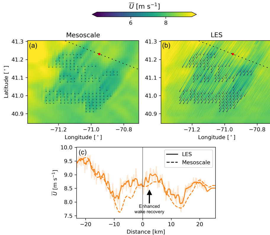
Figure 10. Time-averaged velocity field at hub height for the mesoscale simulation (a) and LES (b) under unstable atmospheric conditions. The velocity fields are averaged in time between 22:00 and 22:15 UTC on 27 July 2017. The dotted black lines in each panel illustrate the locations of the velocity transects, and the red dots indicate the midpoint distance of each transect. Panel (c) shows the velocity along the transect for the LES and mesoscale simulation. For reference, the mean wind direction across the region is 208°.
