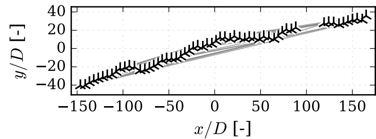
(d) single string, n_{wt} = 58 , s_{wt} = 5.3D
