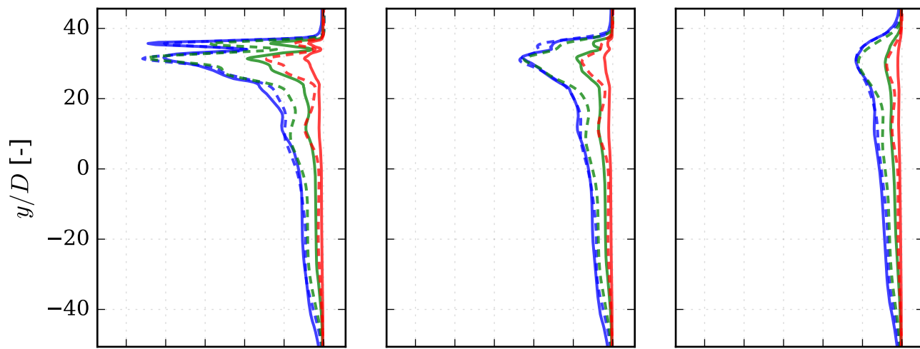
(d) single string, n_{wt} = 58 , s_{wt} = 5.3D
