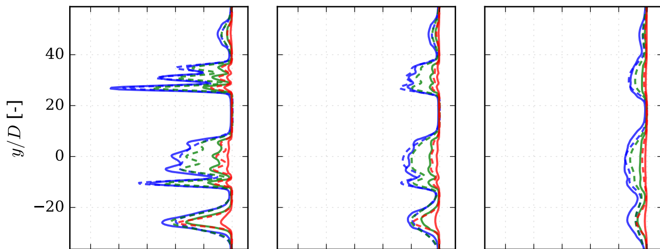
(b) multiple string, n_{wt} = 23 , s_{wt} = 6.0D
