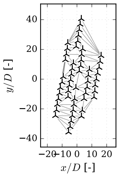
(c) parallel string, n_{wt} = 54 , s_{wt} = 3.7D
