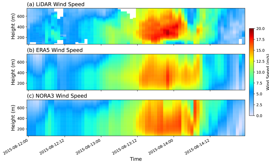
Figure 2. Time–height cross-section of wind speed at FINO1 from different data sources from 12 to 14 August 2015. The times shown in the plots are given in UTC. (a) Lidar observations, (b) ERA5 reanalysis, and (c) NORA3 hindcast.
