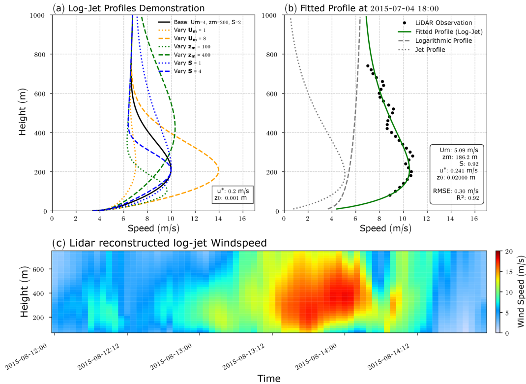
Figure 3. (a) Idealized log-jet profiles illustrating the effect of varying jet parameters. (b) Fitted profiles for lidar observations at 18:00 UTC on 4 July 2015, with the logarithmic and jet components displayed separately. (c) Time–height cross-section of the reconstructed wind speed derived from the fitted log-jet parameters of the lidar data for the same period as in Fig. 2.
