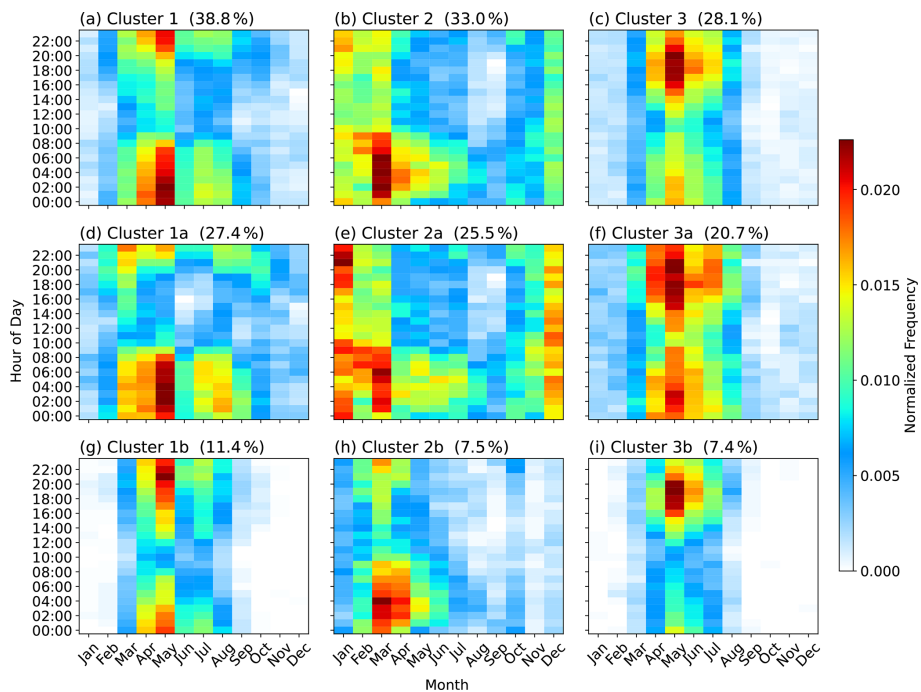
Figure 10. Temporal patterns of LLJ clusters and sub-clusters. The top row (a–c) shows the normalized frequency for the three main clusters, while the second (d–f) and third (g–i) rows display the normalized frequency for sub-clusters a and b, respectively. The times shown in the plots are in UTC.
