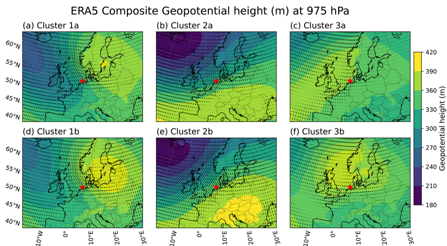
Figure 12. Composite geopotential height (shading, in meters) on the 975 hPa isobaric surface for the same six sub-clusters as in Fig. 9, derived from ERA5 reanalysis. The red star marks the location of the FINO1 offshore station.
