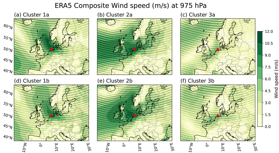
Figure 11. Composite wind speed (shading, in \text{m s}^{-1} ) and wind vectors on the 975 hPa isobaric surface for six sub-clusters derived from ERA5 reanalysis. The red star marks the FINO1 offshore station.
