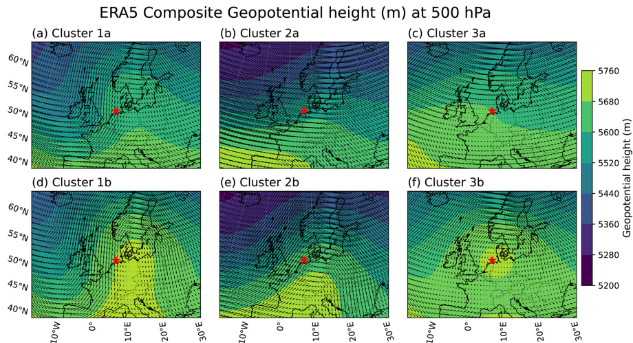
Figure 13. Similar to Fig. 12 but for the 500 hPa isobaric surface.
