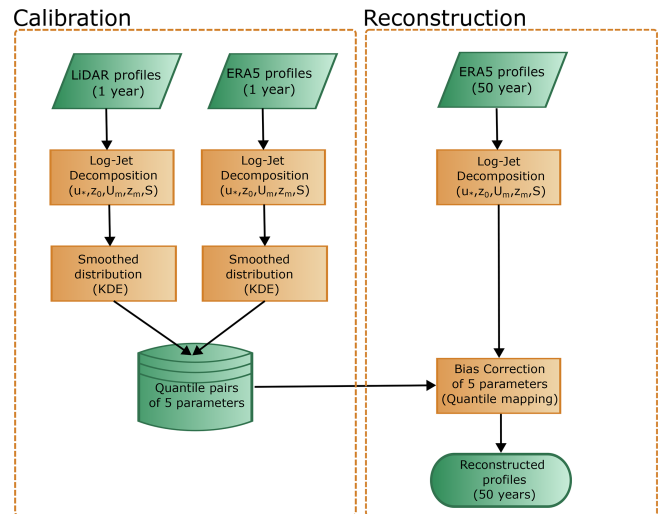
Figure 4. Schematic workflow of the bias correction of the ERA5 wind profiles in this study. The log-jet decomposition allows for model evaluation and provides the basis for the parameter-centric bias correction of the 50-year ERA5 dataset, leading to the LLJ climatology and clustering analysis.
