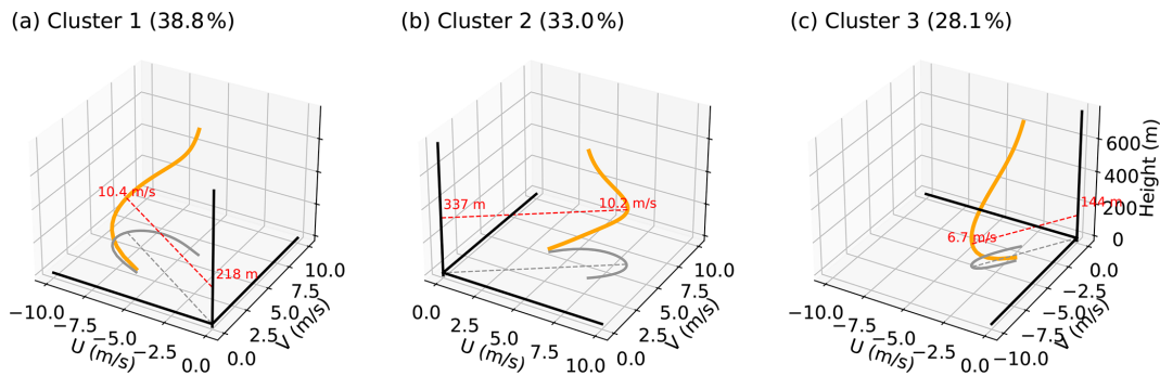
Figure 8. Three-dimensional hodographs of the average wind profiles for the three LLJ clusters. The orange lines represent the mean wind vector, while the thin gray lines on the bottom plane illustrate the horizontal wind projection.
