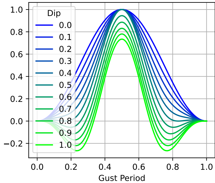
Gust Magnitude
