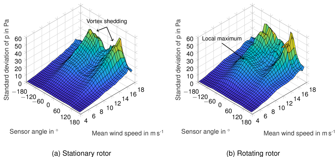
Figure 19. The 1 min averages of the standard deviation of pressure p as a function of sensor angle relative to the wind direction (see Fig. 4 for angle definition) and wind speed. (a) Stationary rotor, when no blade is in front of the tower. (b) Rotating rotor.
