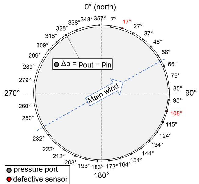
Figure 3. Distribution of pressure ports on the belt in the earth-fixed coordinate system ( 0^\circ facing north). The differential pressure is measured between the tower surface ( p_{\text{out}} ) and the inside of the tower ( p_{\text{in}} ). Two defective sensors (marked in red) were excluded from the analysis.
