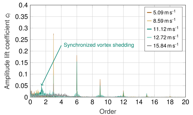
Figure 17. Order-based FFT analysis of the lift coefficient.
