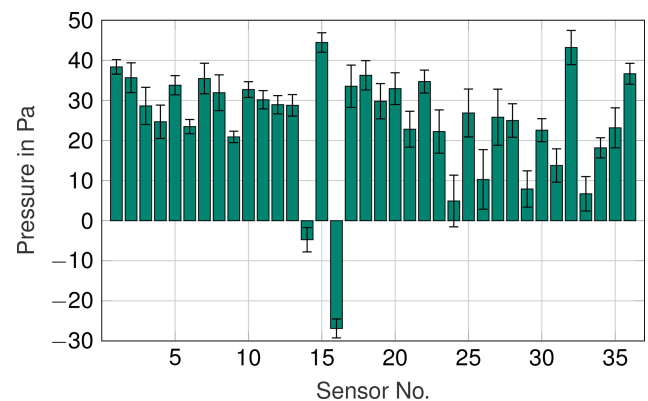
Figure 6. Zero pressure offsets of all 36 pressure sensors. The error bars indicate the measurement uncertainty in the 95 % confidence interval.
