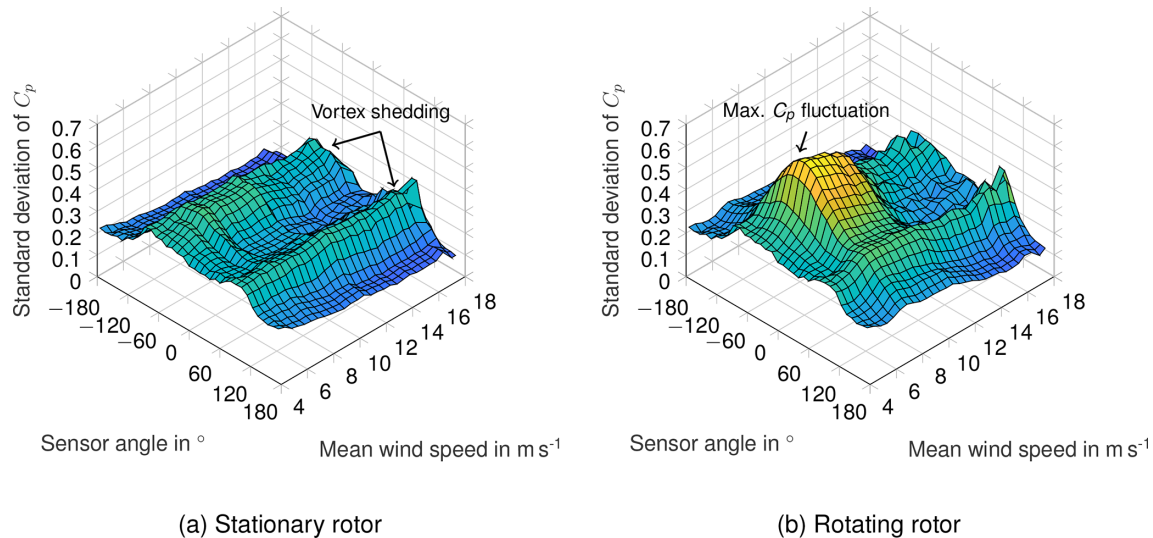
Figure 18. The 1 min averages of the standard deviation of C_p as a function of sensor angle relative to the wind direction (see Fig. 4 for angle definition) and wind speed. (a) Stationary rotor, when no blade is in front of the tower. (b) Rotating rotor.
