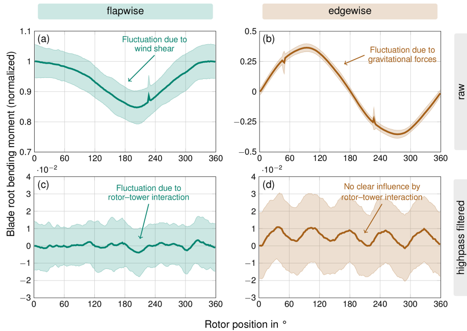
Figure 20. Flapwise (left column) and edgewise (right column) root bending moments of one rotor blade as a function of rotor position for the operating point U_\infty = 11.12 \text{ m s}^{-1} (Table 1). The top row shows the raw signal, while the bottom row shows the high-pass-filtered signal. For confidentiality reasons, the data were normalized to the maximum flapwise bending moment. The shaded areas indicate the standard deviation of the 10 min average.
