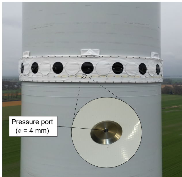
Figure 1. Pressure belt installed on the tower of OPUS 1. The pressure ports have a diameter of 4 mm. A total of 72 pressure ports are integrated into the belt, of which 36 (every second port) were equipped with sensors for this measurement campaign. The black markers are used for digital image correlation (DIC) measurements and were not considered in this study. Photo credit: Kevin Gnebner, DLR.
