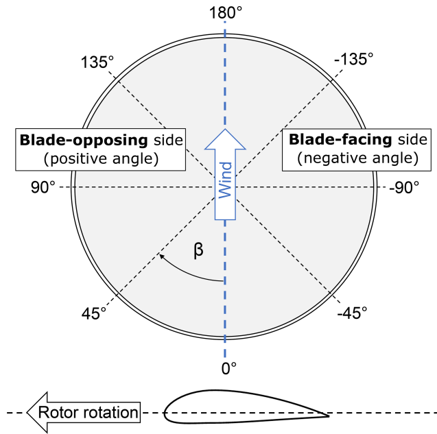
Figure 4. Definition of angle conventions for pressure signals aligned with the wind direction: wind is assumed to come from 0°. The blade passes the tower from right to left. A negative angle \beta corresponds to the blade-facing side, while a positive angle corresponds to the blade-opposing side.
