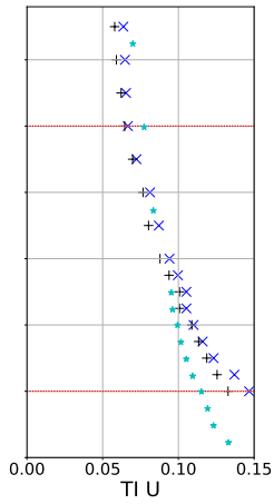
(b) Inlet I_U
