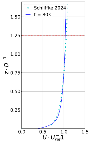
(a) Inlet average velocity
