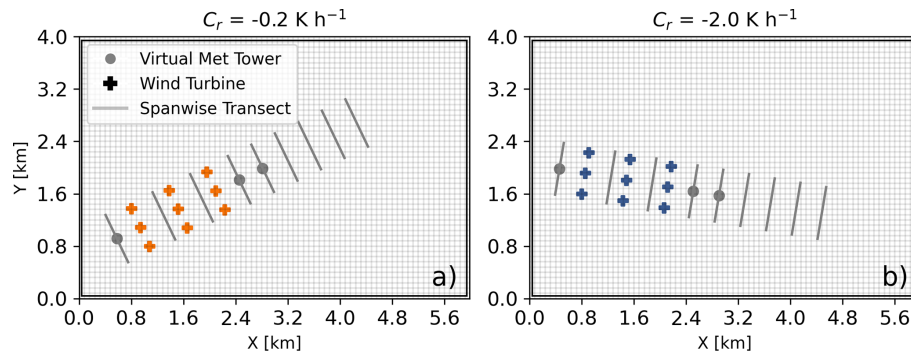
Figure 1. Simulation setup for the (a) weakly and (b) strongly stable regimes denoted by the surface cooling rate C_r . The virtual meteorological tower is located 5D upwind of the wind farm, and the lines represent 10D -wide transects at various locations upwind, within, and downwind of the wind farm.
