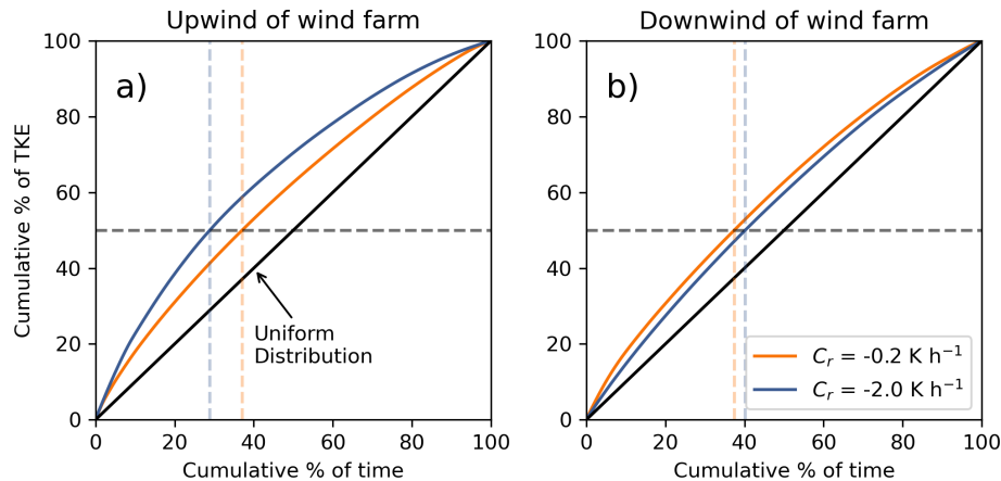
Figure 11. Cumulative distribution function of TKE (a) 5D upwind ( x = -5D ) and (b) 10D downwind ( x = 26D ) of the wind farm for each stability regime at z = 50 m. The dashed lines pinpoint the cumulative percentage of time it takes until 50 % of the TKE occurs.
