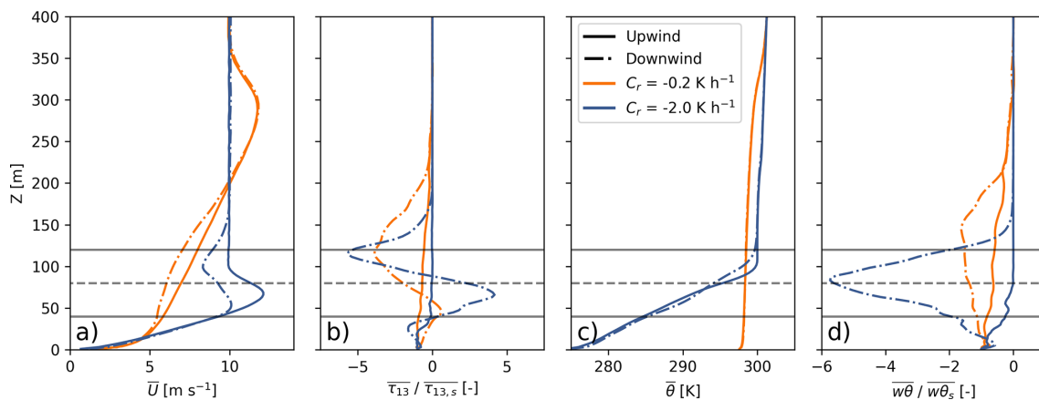
Figure 12. Vertical profiles of (a) wind speed, (b) streamwise vertical momentum flux, (c) potential temperature, and (d) vertical heat flux 5D upwind ( x = -5D ) and 5D downwind ( x = 21D ) of the farm for each stability regime. The solid horizontal lines represent the bottom and top of the rotor layer, while the dashed line represents hub height.
