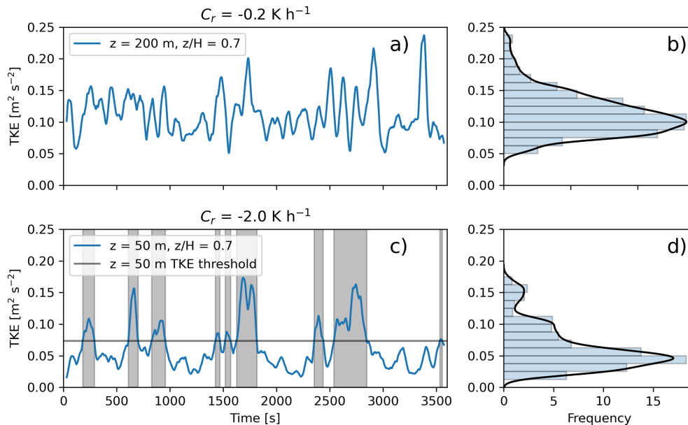
Figure 7. Time series of TKE at 70 % of the boundary layer height for the (a) weakly and (c) strongly stable regimes. Histogram of the TKE distribution for the (b) weakly and (d) strongly stable regimes. The black lines in (b) and (d) represent kernel density estimates of the probability distribution functions. In (c), the periods highlighted in gray are “turbulent”, while other periods are “quiescent”.
