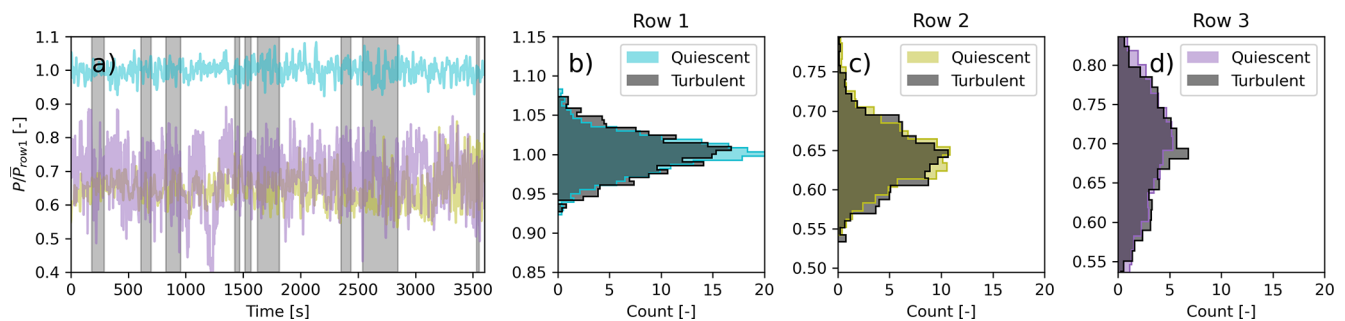
Figure 16. Time series (a) and histograms by row (b–d) of detrended power normalized by the rated power of the turbine for the strongly stable regime. The periods highlighted in gray are turbulent, while periods in white are quiescent, as determined by the method in Sect. 3.2.
