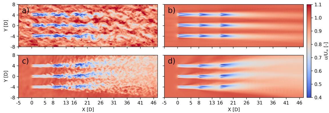
Figure 9. Instantaneous (a, c) and 1 h time-averaged (b, d) plan view of velocity deficits at hub height for the weakly (a, b) and strongly (c, d) stable regimes.
