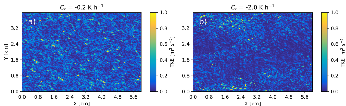
Figure 8. Instantaneous plan view of TKE at the beginning of the analysis period for the (a) weakly stable regime at 200 m a.g.l. and (b) strongly stable regime at 50 m a.g.l. Note that both heights correspond to 70 % of the boundary layer height for each regime.
