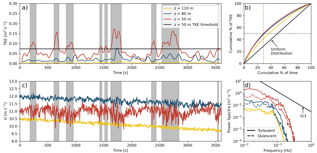
Figure 6. (a) Time series and (b) cumulative distribution function of TKE at various heights within the rotor disk for the strongly stable regime 5D upwind of the wind farm on the inner domain. (c) Time series and (d) power spectra of wind speed at the same heights as in (a) and (b). The dashed lines in (b) pinpoint the cumulative percentage of time it takes until 50 % of the TKE occurs at a height of 50 m. The periods highlighted in gray are “turbulent”, while other periods are “quiescent”. In (d), the -5/3 inertial subrange power law is provided in black for reference.
