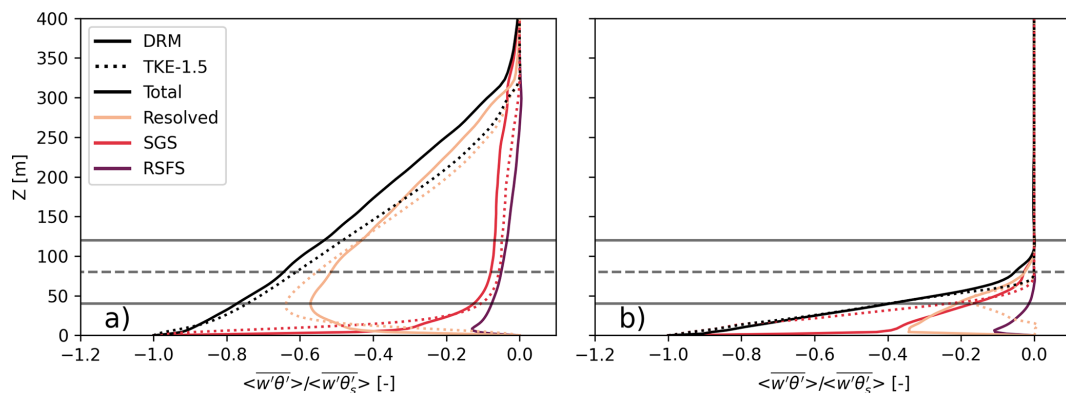
Figure 3. Planar- and time-averaged vertical profiles of normalized heat flux for the (a) weakly stable and (b) strongly stable regime for the DRM and TKE-1.5 closures at 8 m resolution. Note that the results shown are for the outer domain without wind turbines. The solid horizontal lines represent the bottom and top of the rotor layer, while the dashed line represents hub height.
