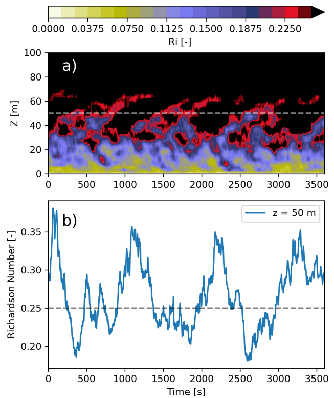
Figure B1. (a) Time–height contour of the gradient Richardson number ( Ri ) at 5D upwind of the wind farm on the inner domain during the analysis period emphasizing the critical Richardson number value of 0.25. (b) Time series of Ri at z = 50 m with a dashed line at Ri = 0.25 corresponding to the critical Richardson number.
