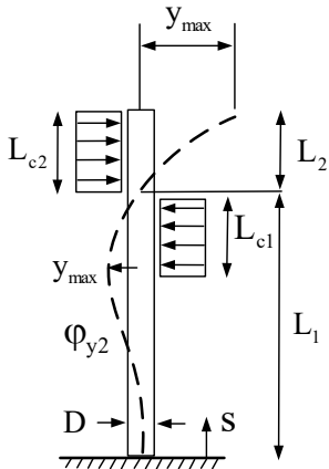
2 nd mode shape
