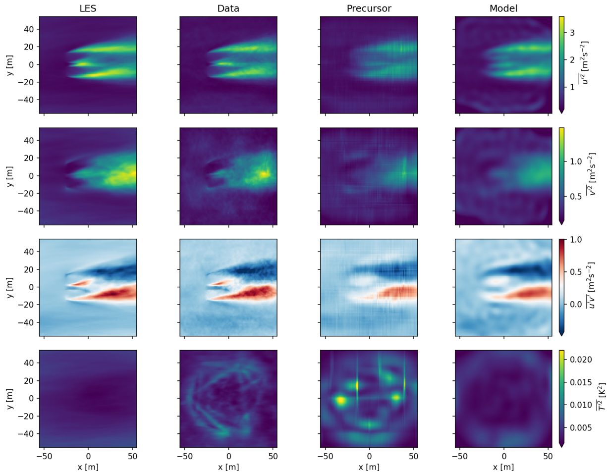
Figure 15. Comparison of the simulated streamwise and spanwise Reynolds normal stresses, the in-plane Reynolds shear stress, and the temperature variance (from top) to the AT retrievals for the convective case.
