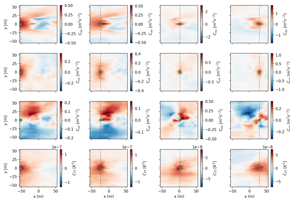
Figure A3. Examples of the correlation functions for the neutral wind turbine wake case. The central point ( r ) for each plot is indicated with a green marker. Vertical dashed gray lines indicate transects for which profiles are compared in Fig. 12.
