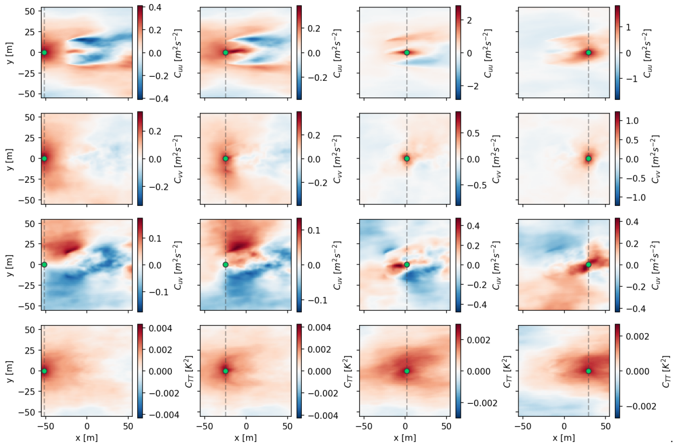
Figure 10. Examples of the correlation functions for the convective wind turbine wake case. The central point ( r ) for each plot is indicated with a green marker. Vertical dashed gray lines indicate transects for which profiles are compared in Fig. 12.
