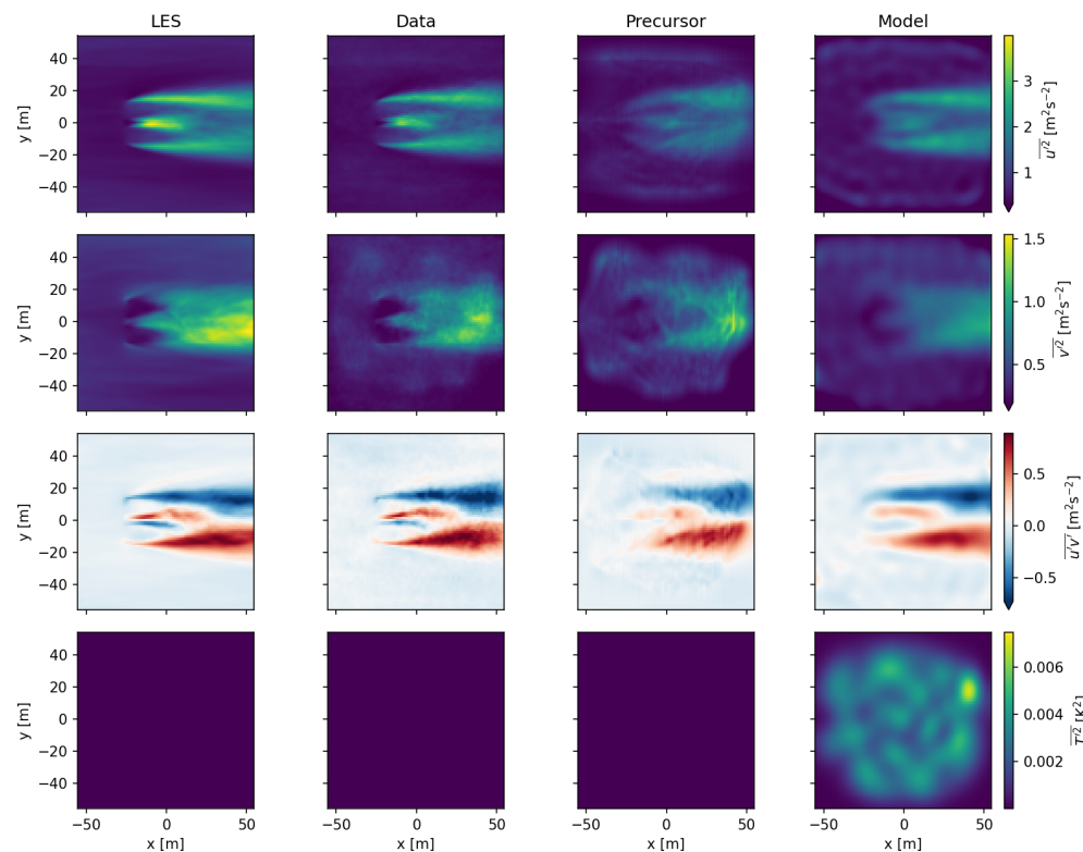
Figure A4. Comparison of the simulated variances of the streamwise and spanwise velocity components, their covariance, and the variance of temperature (from top) to the AT retrievals for the neutral case.
