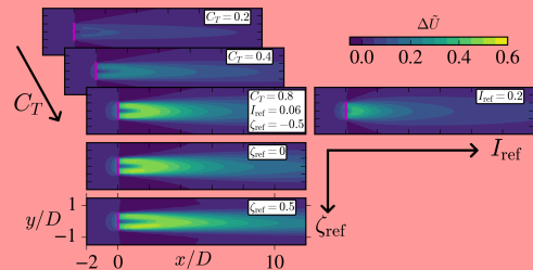
a) Velocity deficit, \Delta\tilde{U}
