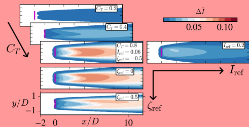
b) Wake-added TI, \Delta\tilde{I}
