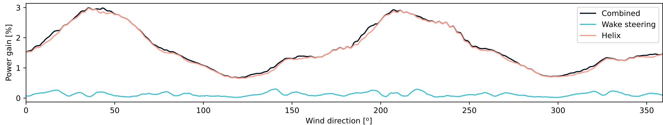
Wind direction uncertainty: \sigma_\theta = 5^\circ
