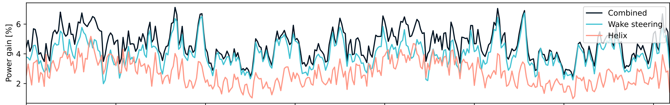
Wind direction uncertainty: \sigma_\theta = 2.5^\circ
