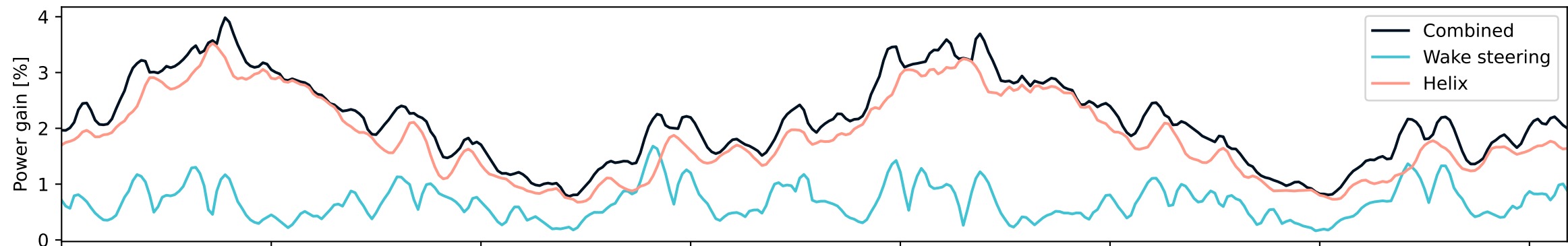
Wind direction uncertainty: \sigma_\theta = 5^\circ
