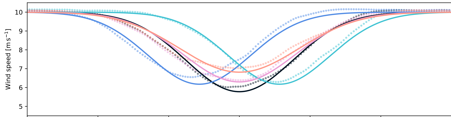
Downstream distance: 6.0 D
