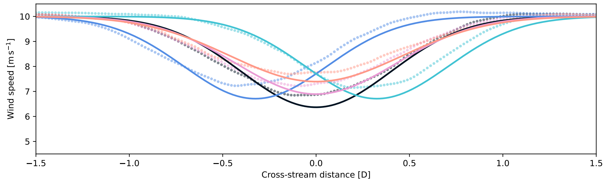
Downstream distance: 8.0 D
