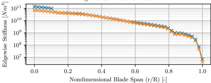
Edgewise Stiffness Distribution
