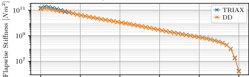
Flapwise Stiffness Distribution
