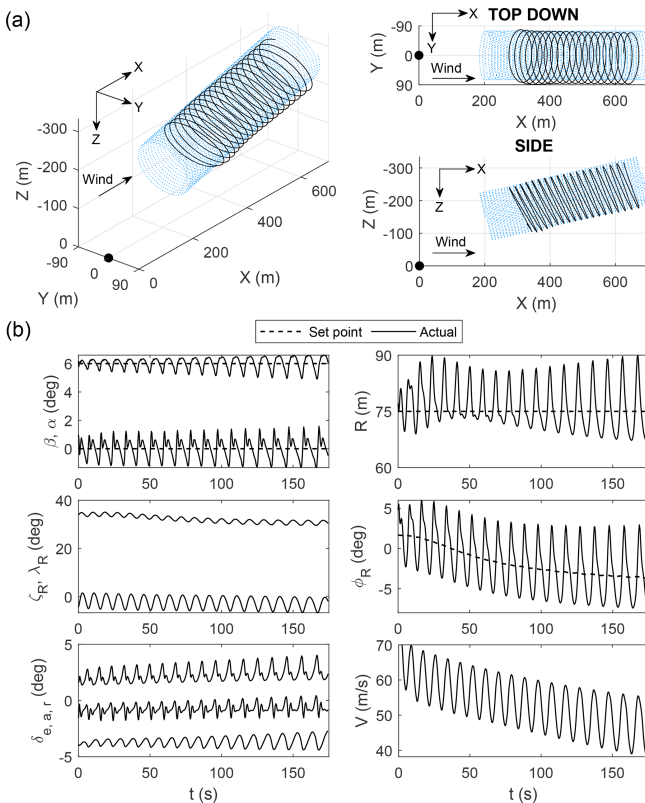
Figure 13. A typical circular reel-out trajectory with parameters \mathbf{P} = [200, 0, -150] m, [\lambda_p, \zeta_p] = [13^\circ, 0^\circ] , and R_{sp} = 75 m. The winch speed is kept constant at 2.0 \text{ m s}^{-1} .
