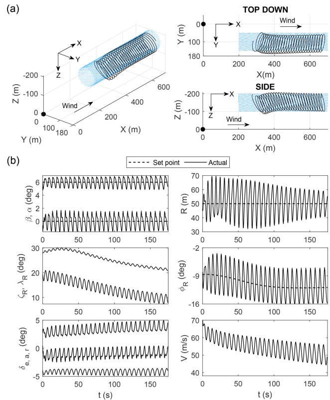
Figure 15. Sideway reel out with parameters \mathbf{P} = [200, 100, -150] \text{ m} , [\lambda_P, \zeta_P] = [0^\circ, 0^\circ] , and R_{SP} = 50 \text{ m} . The winch speed is kept constant at 2.0 \text{ m s}^{-1} .
