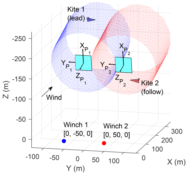
Figure 31. Starting location of the two kites for synchronisation testing.
