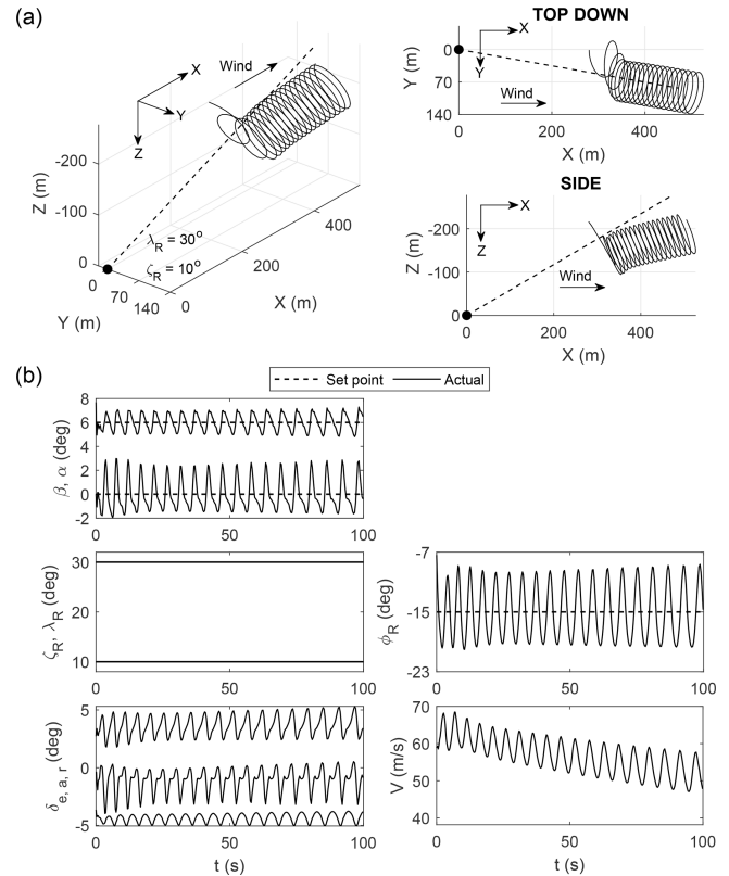
Figure 26. Semi-manual flight using only the inner loop.
