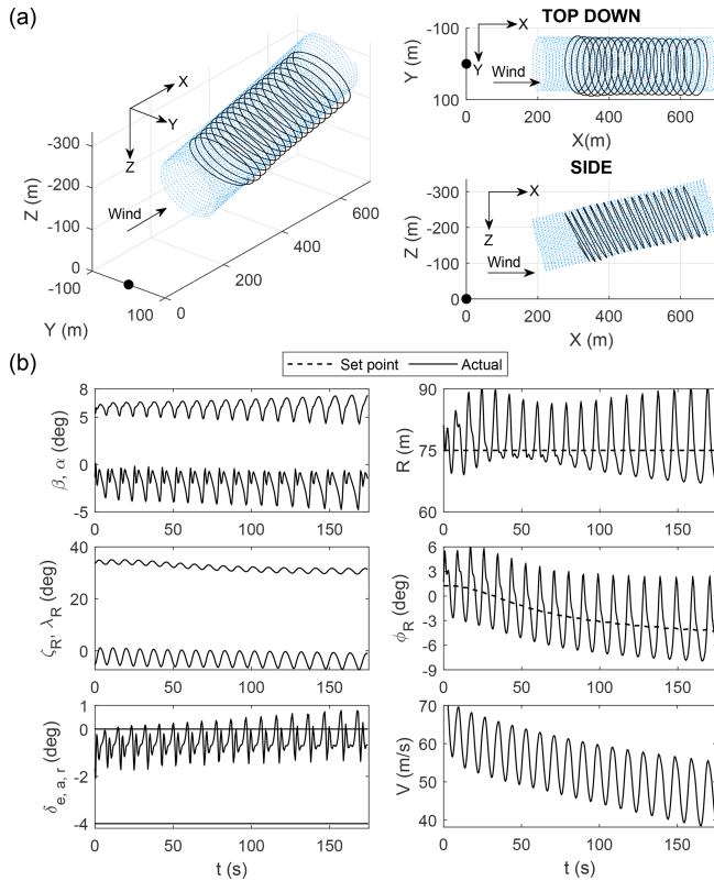
Figure 25. Normal reel out flown with fixed elevator ( -4^\circ ) and rudder ( 0^\circ ). Parameters: \mathbf{P} = [200, 0, -150] m, [\lambda_P, \zeta_P] = [13^\circ, 0^\circ] , and R_{SP} = 75 m. The winch speed is kept constant at 2.0 \text{ m s}^{-1} .
