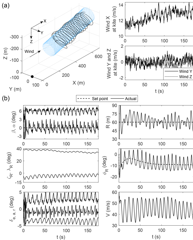
Figure 19. Reel out in medium wind and medium turbulence. The winch speed is kept constant at 2.0 \text{ m s}^{-1} . A better tracking performance can be achieved by reducing the winch speed.
