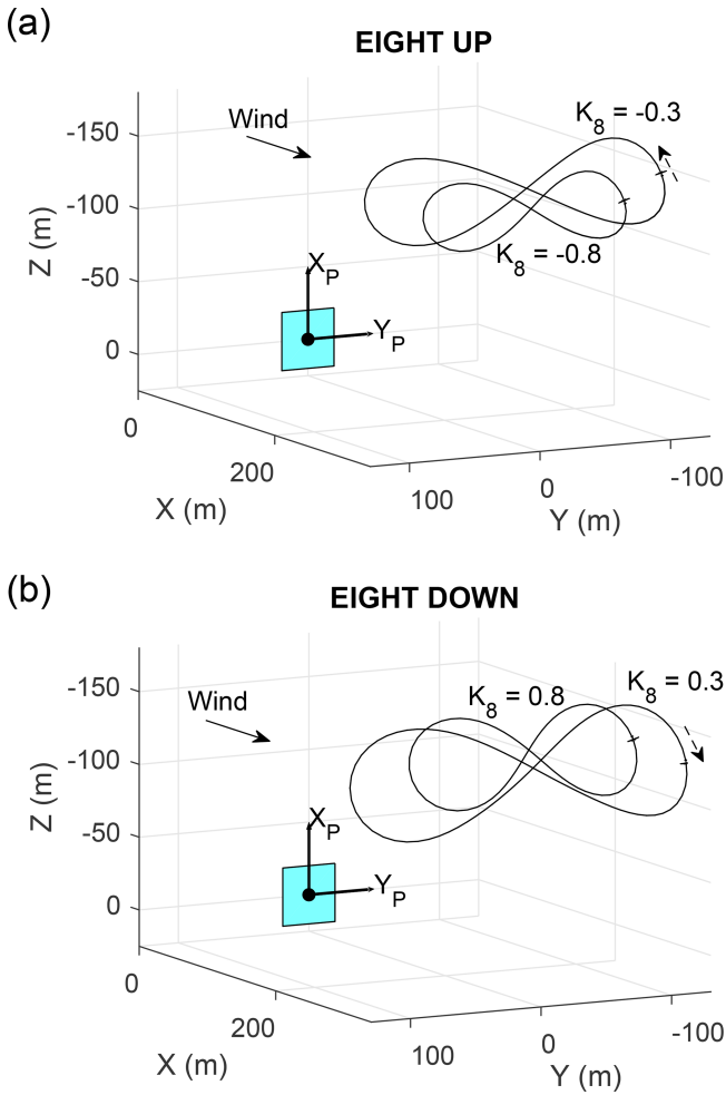
Figure 36. Eight-up (a) and eight-down (b) trajectories at \lambda_R = 25^\circ with different control gains.
