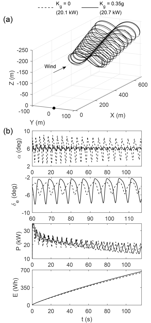
Figure 38. Eight-down reel out without and with \alpha -suppression control.
