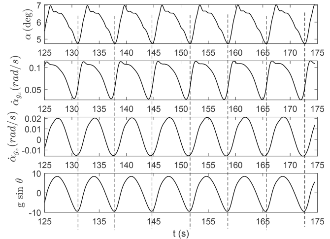
Figure 28. Potential feedback terms to cancel out the effect of gravity on \alpha oscillation.
