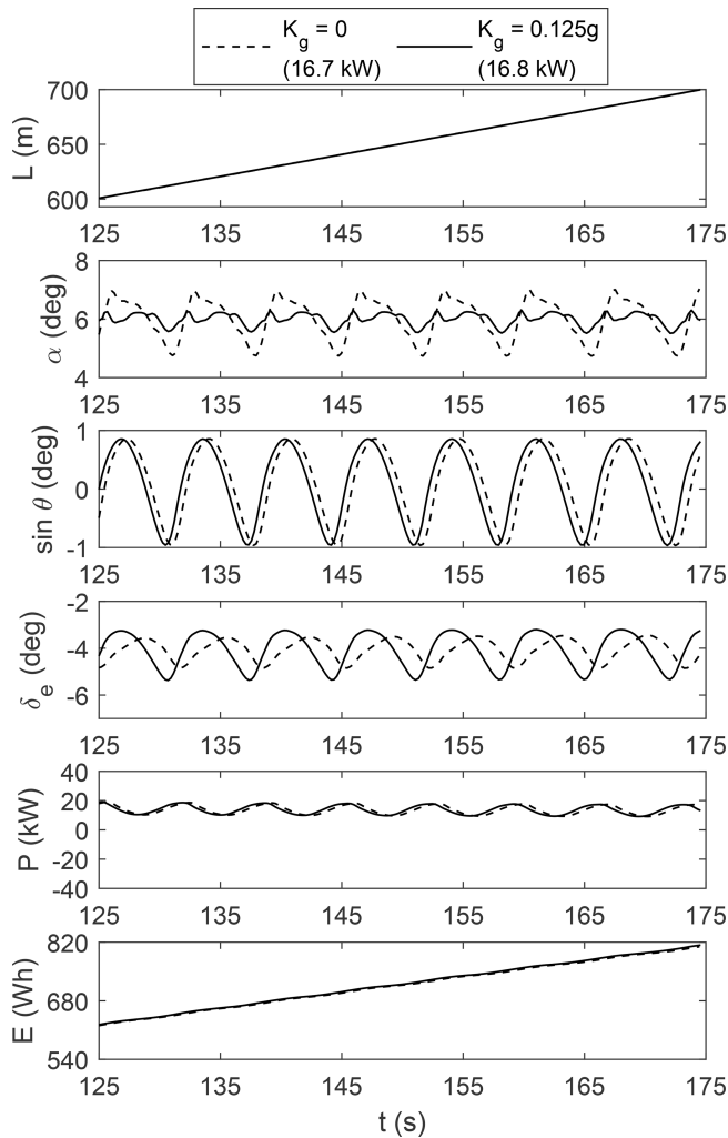
Figure 29. Effect of the \alpha -suppression controller. The winch speed is constant at 2 \text{ m s}^{-1} .
