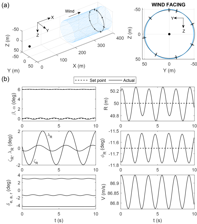
Figure 27. Closed-loop limit cycles, which is always present in the full flight controller even when equilibrium trim is possible.
