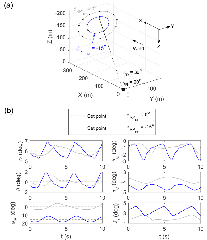
Figure 10. Closed-loop trajectories (a) and time histories (b) with different \phi_{RSP} . The kite is drawn true to scale at 0.5 s intervals.
