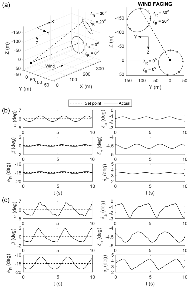
Figure 8. Closed-loop trajectories (a) and time histories (b and c) with two different reference plane orientations. The time histories of [\lambda_R, \zeta_R] = [0^\circ, 0^\circ] and [\lambda_R, \zeta_R] = [30^\circ, 20^\circ] are shown in (b) and (c), respectively.
