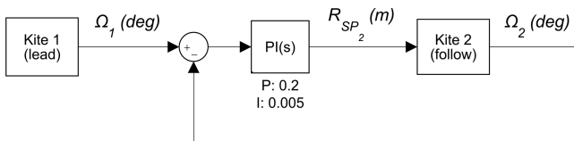
Figure 32. Phase synchronisation controller in the second kite.
