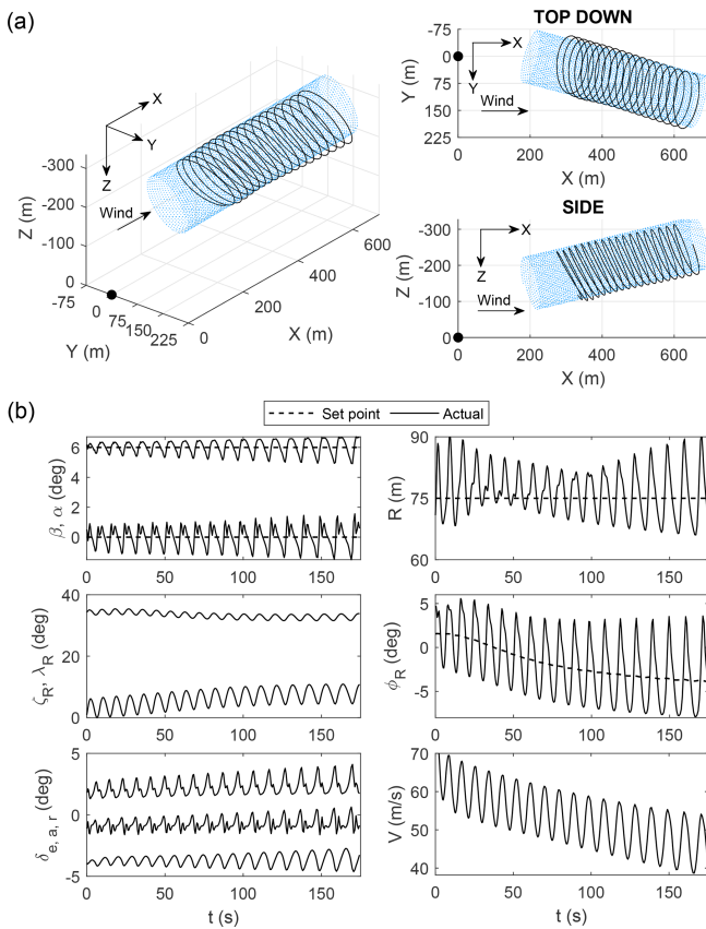
Figure 14. Diagonal reel out with parameters \mathbf{P} = [200, 0, -150] \text{ m} , [\lambda_P, \zeta_P] = [13^\circ, 15^\circ] , and R_{SP} = 75 \text{ m} . The winch speed is kept constant at 2.0 \text{ m s}^{-1} .
