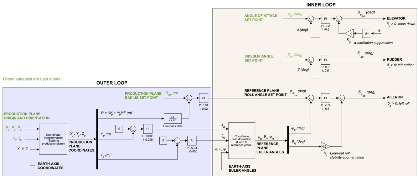
Figure 12. Full flight control system. The Earth-to-production-plane coordinate transformation is presented in Appendix B.
