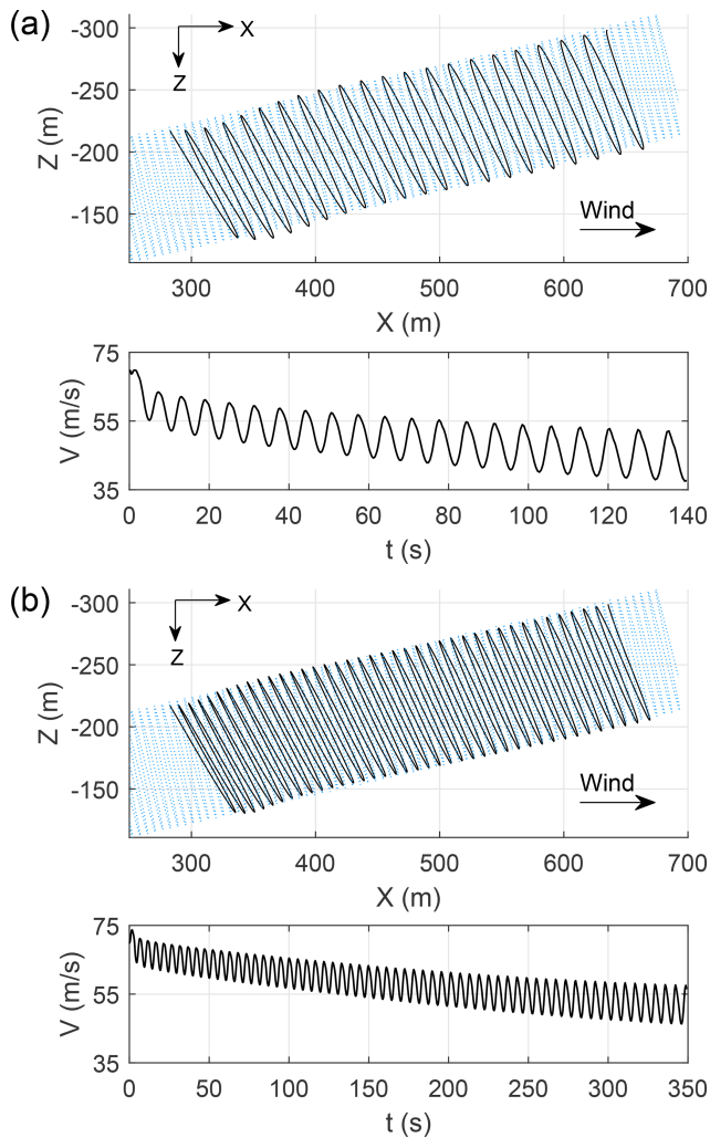
Figure 21. Reeling out at 2.5 \text{ m s}^{-1} (a) and 1.0 \text{ m s}^{-1} (b) wind speed, showing lower airspeed in (a) due to faster reel out.
