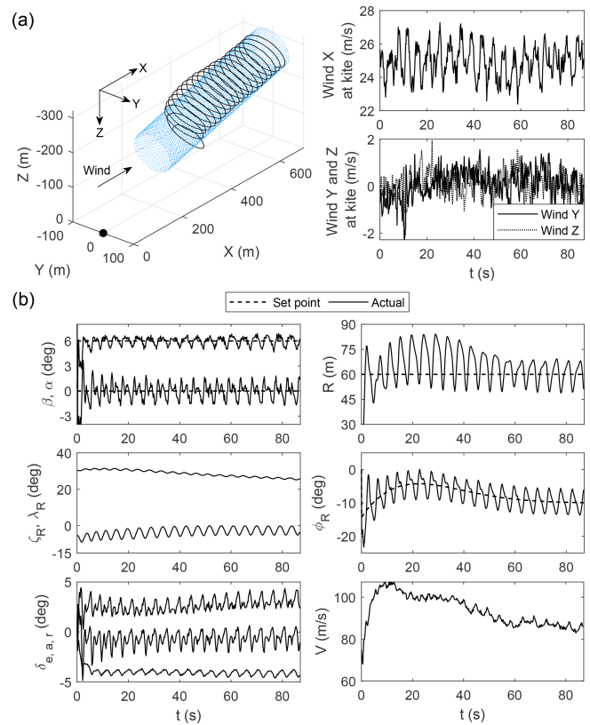
Figure 20. Reel out in high wind and high turbulence. The winch speed is kept constant at 4.0 \text{ m s}^{-1} .
