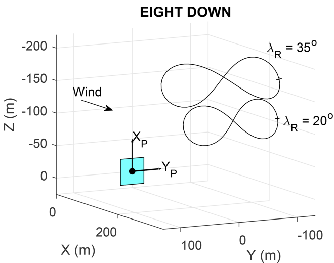
Figure 37. Effect of changing \lambda_R .
