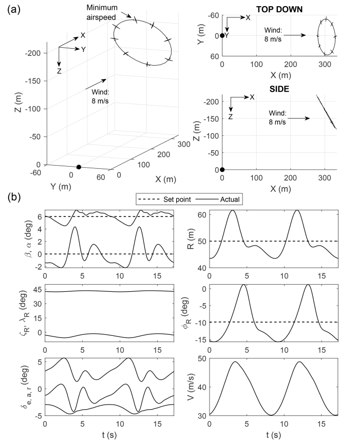
Figure 22. Trajectory under zero winch speed in 8 \text{ m s}^{-1} wind. The kite is drawn true to scale at 1 s intervals. Time histories show data from two cycles.
