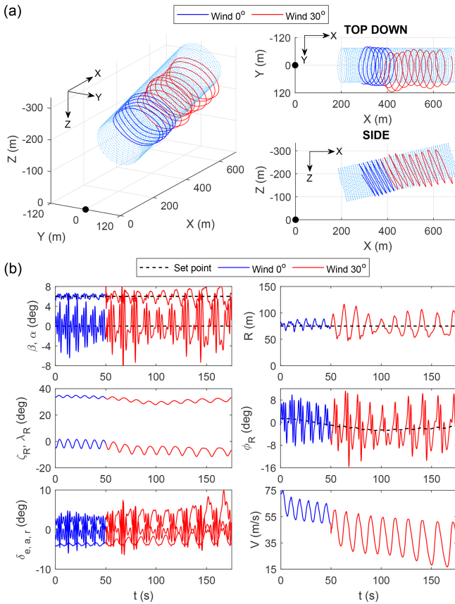
Figure 16. Closed-loop response to a sudden change in wind direction using a discrete controller (10 Hz) with feedback delay (0.1 s) and no corrective action to the target cylinder.
