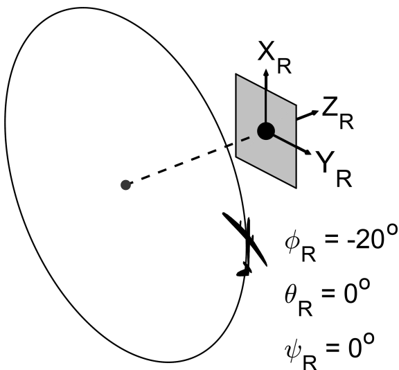
Figure 6. Example left-roll circular orbit as defined by the reference plane.
