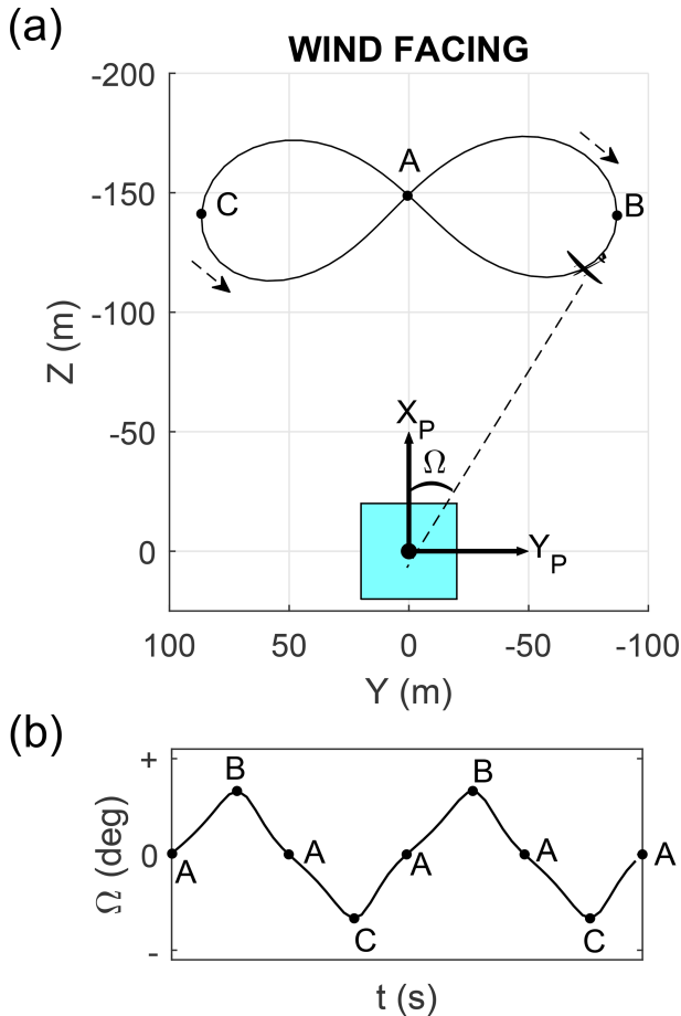
Figure 34. A generic figure-of-eight pattern (a) and evolution of the phase angle over two cycles (b).
