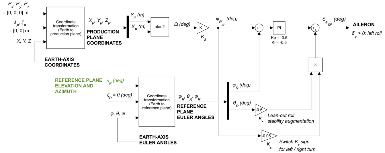
Figure 35. Block diagram of the figure-of-eight flight controller for aileron. Note that the elevator and rudder loops remain unchanged.
